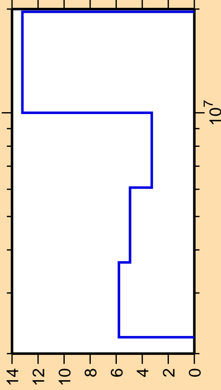
\Delta\sigma/\sigma vs. E for ^{130}\text{Xe}(n,n\text{cont.})
