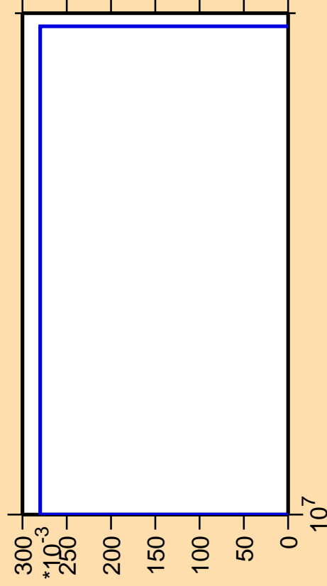
\Delta\sigma/\sigma vs. E for ^{130}\text{Xe}(n,nt)
