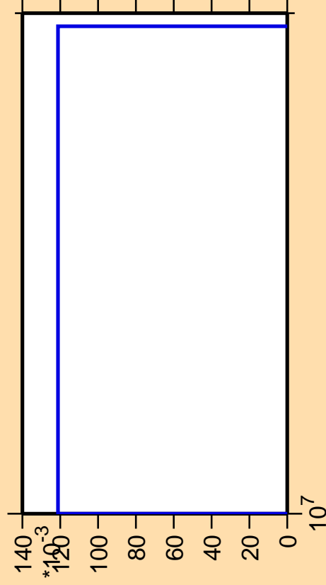
\Delta\sigma/\sigma vs. E for ^{130}\text{Xe}(n,2n\alpha)
