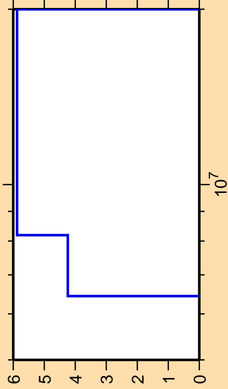
\Delta\sigma/\sigma vs. E for ^{131}\text{Xe}(n,n\text{cont.})
