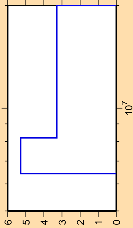
\Delta\sigma/\sigma vs. E for ^{131}\text{Xe}(n,2n)
