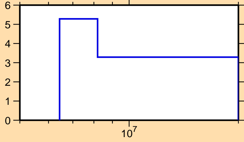
\Delta\sigma/\sigma vs. E for ^{131}\text{Xe}(n,2n)
