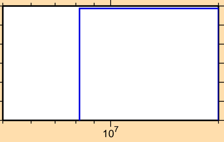
\sigma vs. E for ^{131}\text{Xe}(n,\text{nd})
