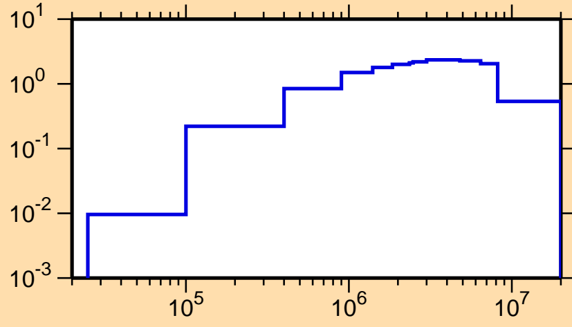
\sigma vs. E for ^{131}\text{Xe}(n,\text{inel.})
