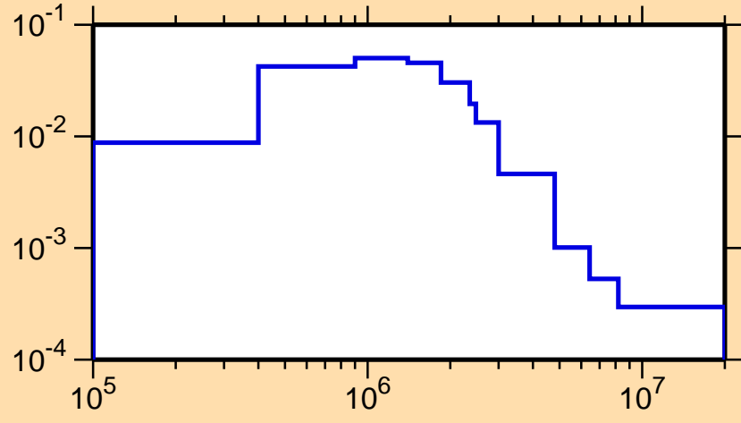
\sigma vs. E for ^{131}\text{Xe}(n,n_2)
