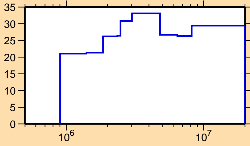
\Delta\sigma/\sigma vs. E for ^{131}\text{Xe}(n,\gamma)
