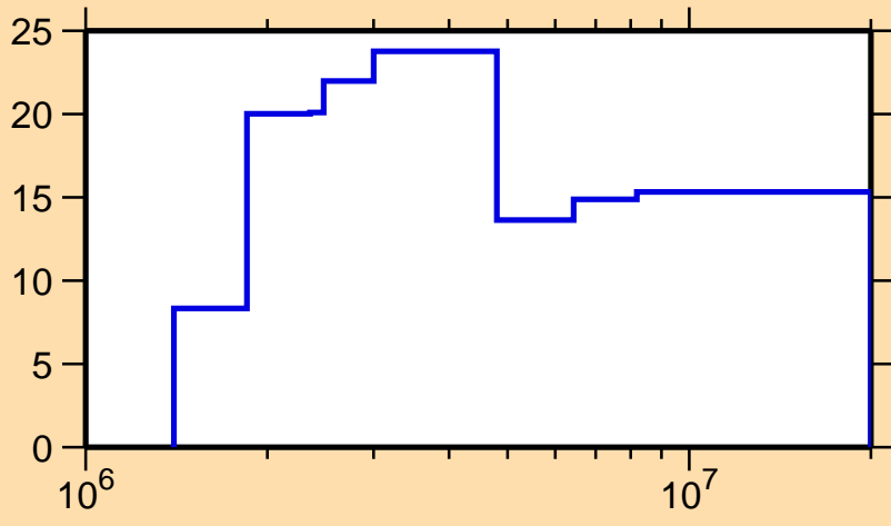
\Delta\sigma/\sigma vs. E for ^{131}\text{Xe}(n,n_1)
