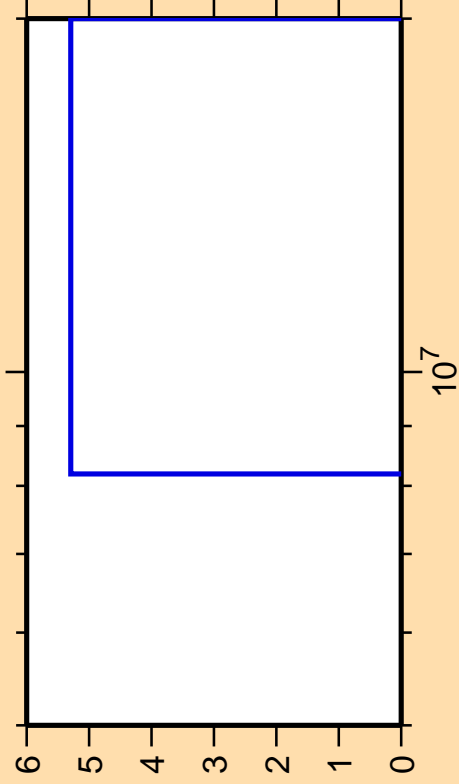
\Delta\sigma/\sigma vs. E for ^{131}\text{Xe}(n,3n)
