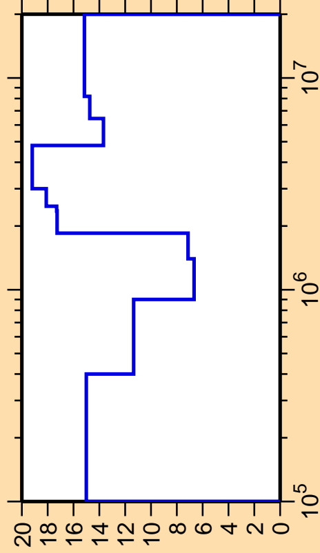
\Delta\sigma/\sigma vs. E for ^{131}\text{Xe}(n,n_2)
