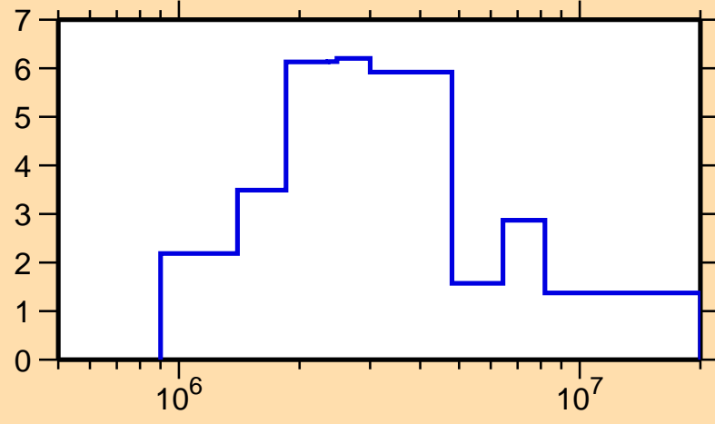
\Delta\sigma/\sigma vs. E for ^{131}\text{Xe}(n,el.)
