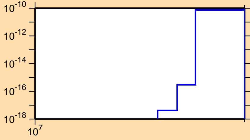
\sigma vs. E for ^{132}\text{Xe}(n,nt)
