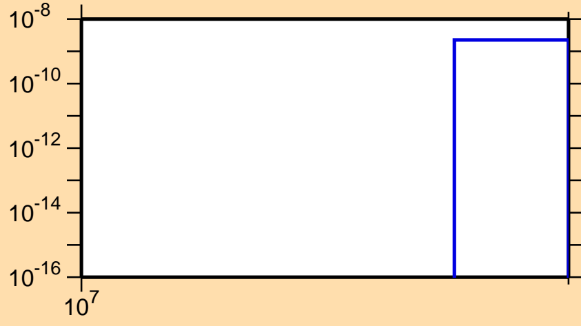
\sigma vs. E for ^{132}\text{Xe}(n,\text{nd})
