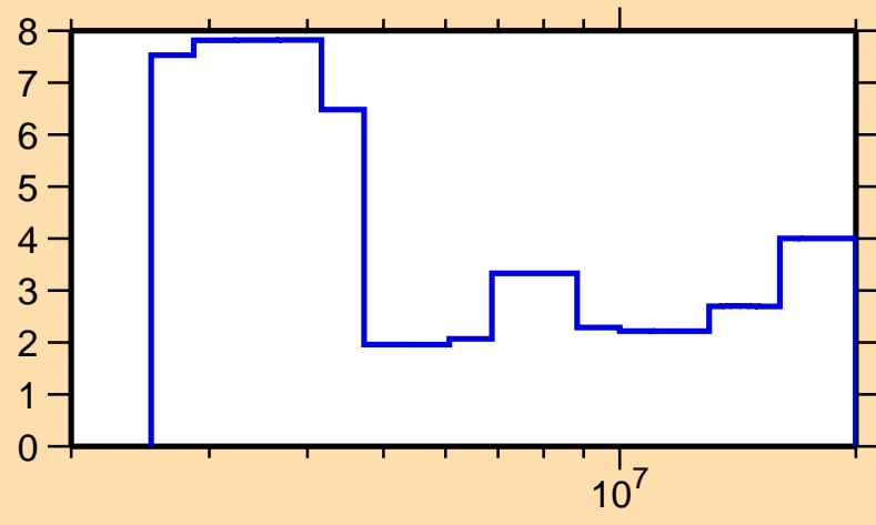
\Delta\sigma/\sigma vs. E for ^{132}\text{Xe}(n, el.)
