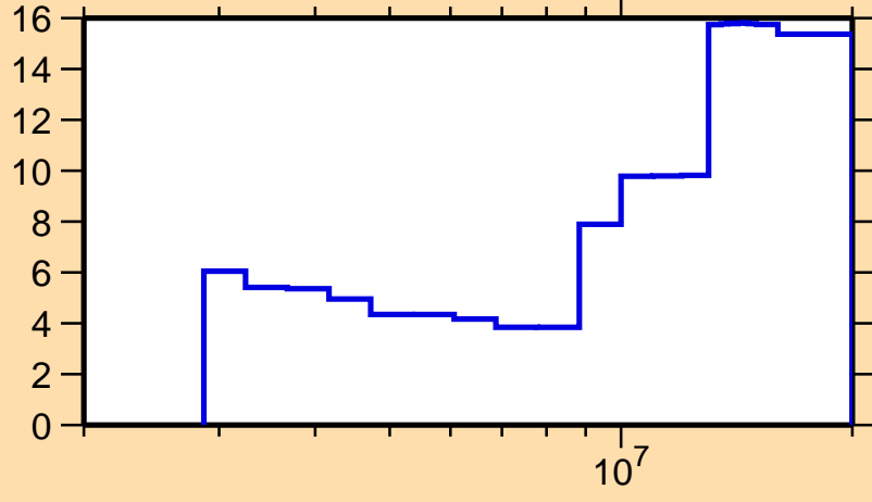
\Delta\sigma/\sigma vs. E for ^{132}\text{Xe}(n,n\text{cont.})
