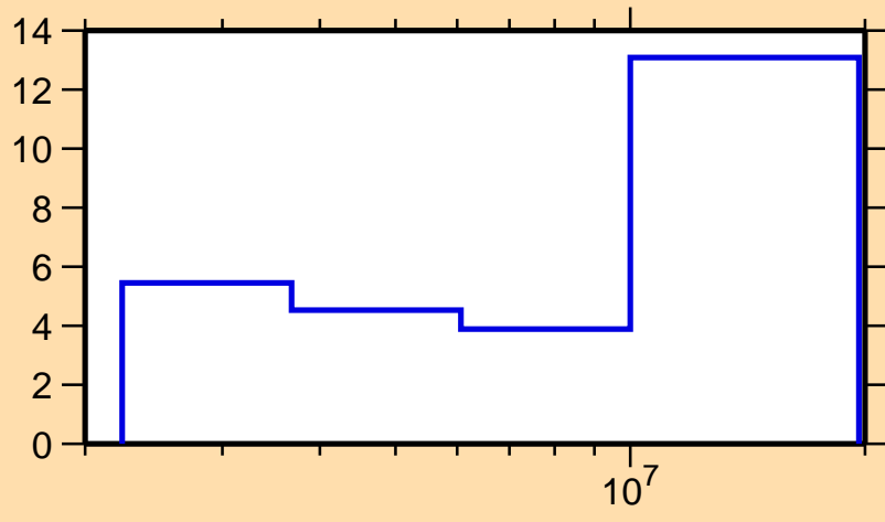
\Delta\sigma/\sigma vs. E for ^{132}\text{Xe}(n, n\text{cont.})
