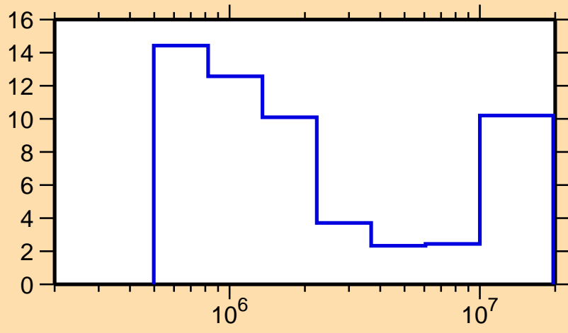
\Delta\sigma/\sigma vs. E for ^{132}\text{Xe}(n,\text{inel.})
