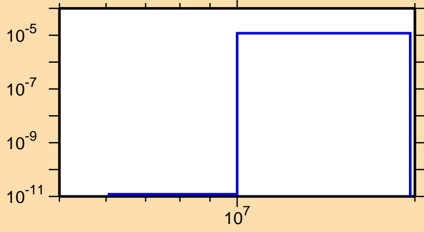
\sigma vs. E for ^{132}\text{Xe}(n,n\alpha)
