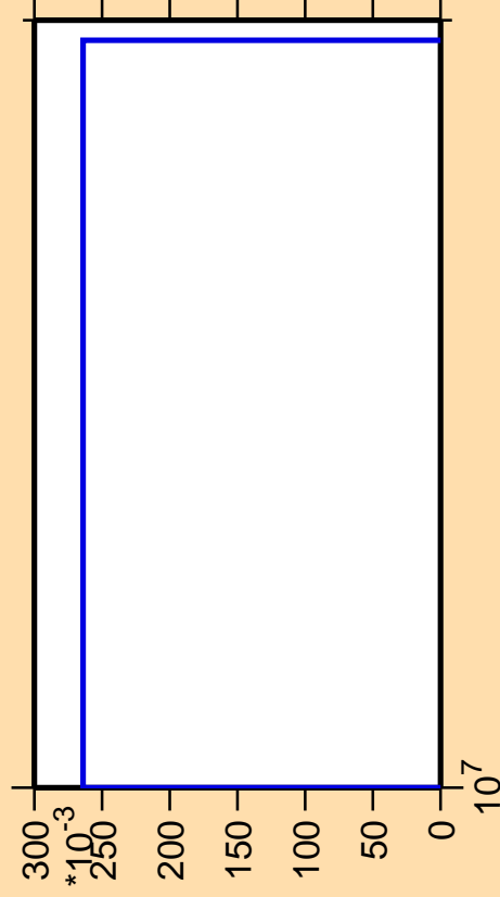
\Delta\sigma/\sigma vs. E for ^{132}\text{Xe}(n,2n\alpha)
