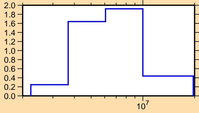
\sigma vs. E for ^{132}\text{Xe}(n,n\text{cont.})
