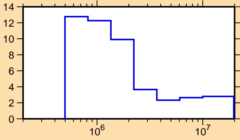
\Delta\sigma/\sigma vs. E for ^{132}\text{Xe}(n,\text{nonel.})
