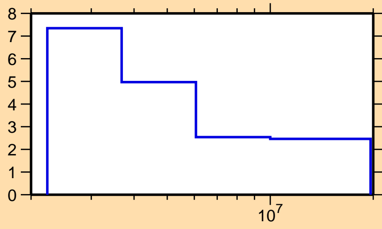
\Delta\sigma/\sigma vs. E for ^{132}\text{Xe}(n,\text{el.})
