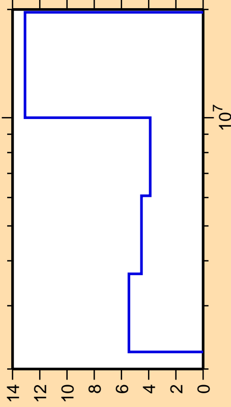
\Delta\sigma/\sigma vs. E for ^{132}\text{Xe}(n,n\text{cont.})
