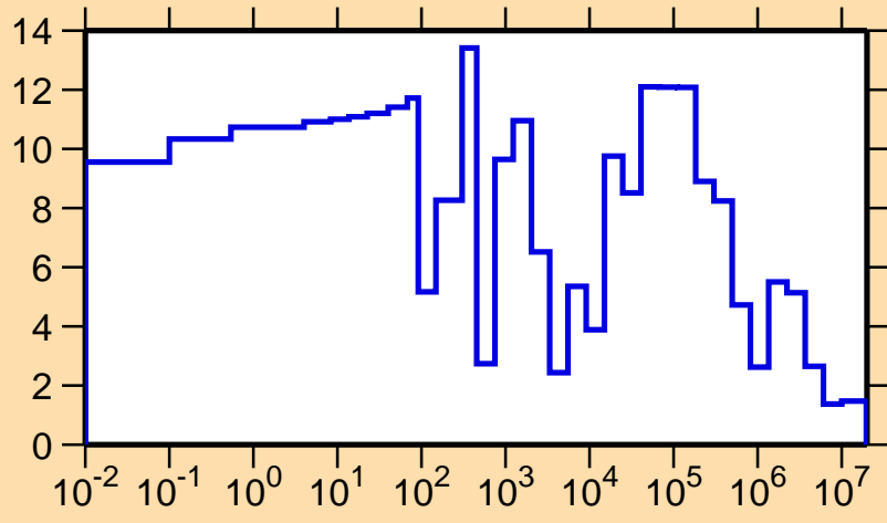
\Delta\sigma/\sigma vs. E for ^{132}\text{Xe}(n,\text{tot.})
