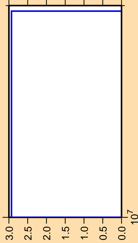
\Delta\sigma/\sigma vs. E for ^{132}\text{Xe}(n,\text{He}3)
