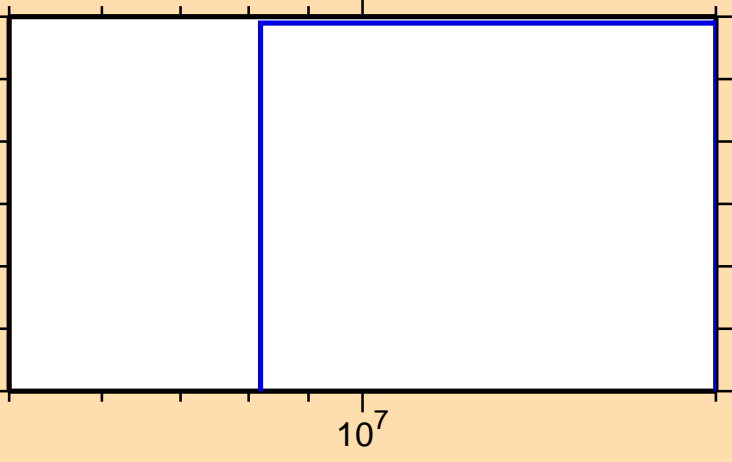
\sigma vs. E for ^{132}\text{Xe}(n,d)
