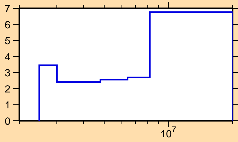
\Delta\sigma/\sigma vs. E for ^{132}\text{Xe}(n,\text{inel.})
