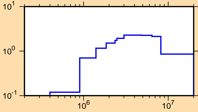
\sigma vs. E for ^{132}\text{Xe}(n,\text{inel.})
