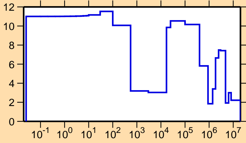
\Delta\sigma/\sigma vs. E for ^{132}\text{Xe}(n,\text{el.})
