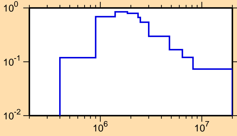
\sigma vs. E for ^{132}\text{Xe}(n,n_1)
