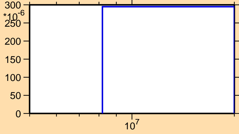
\sigma vs. E for ^{132}\text{Xe}(n,d)
