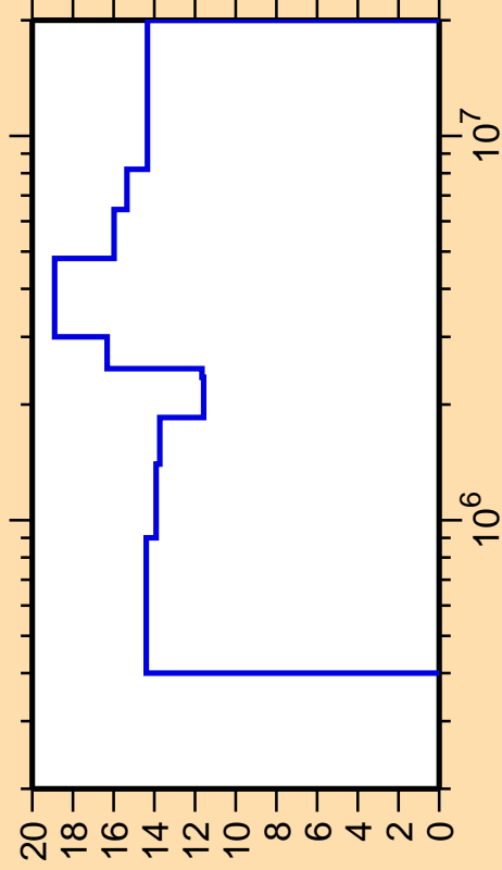
\Delta\sigma/\sigma vs. E for ^{132}\text{Xe}(n,n_1)
