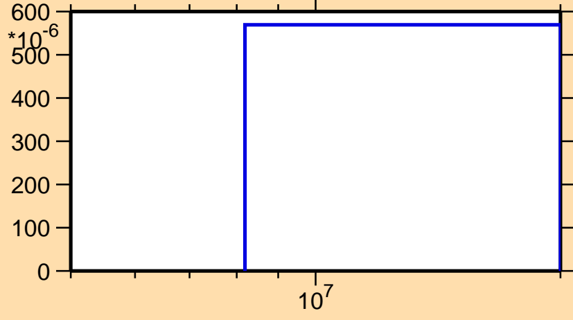
\sigma vs. E for ^{132}\text{Xe}(n,3n)
