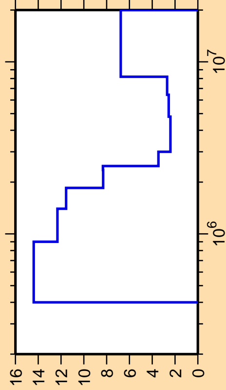
\Delta\sigma/\sigma vs. E for ^{132}\text{Xe}(n,\text{inel.})
