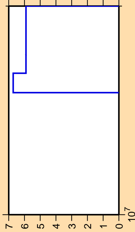
\Delta\sigma/\sigma vs. E for ^{133}\text{Xe}(n,3n)
