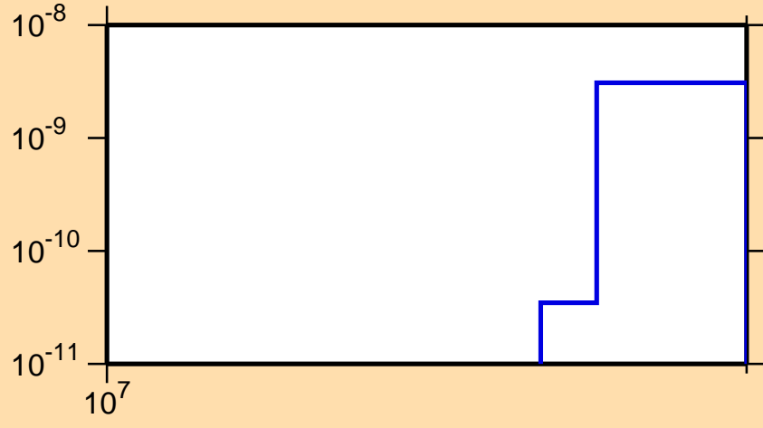
\sigma vs. E for ^{133}\text{Xe}(n,2n\alpha)
