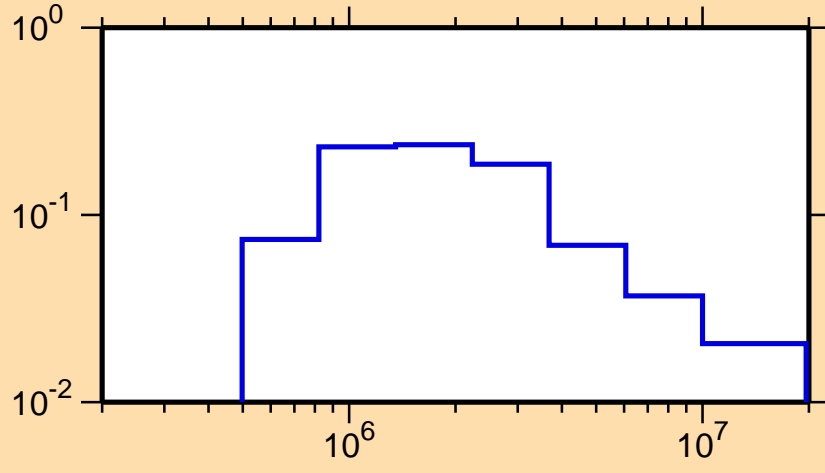
\sigma vs. E for ^{133}\text{Xe}(n,n_4)
