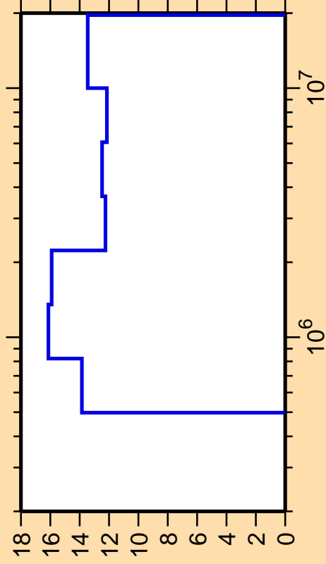
\Delta\sigma/\sigma vs. E for ^{133}\text{Xe}(n,n_4)
