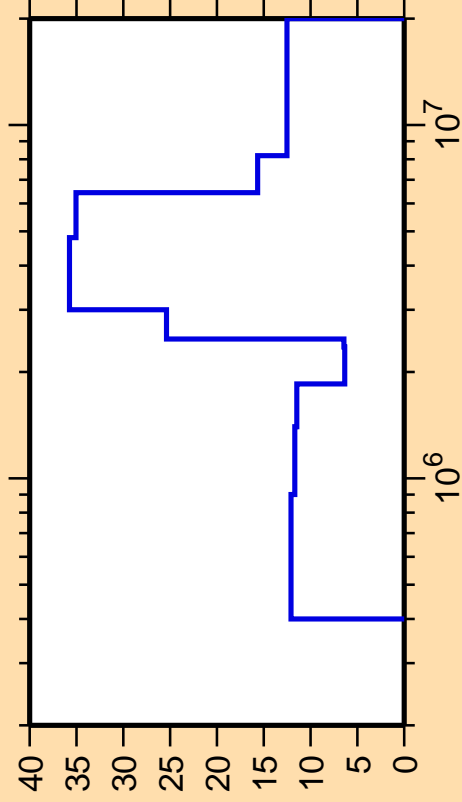
\Delta\sigma/\sigma vs. E for ^{133}\text{Xe}(n,n_3)
