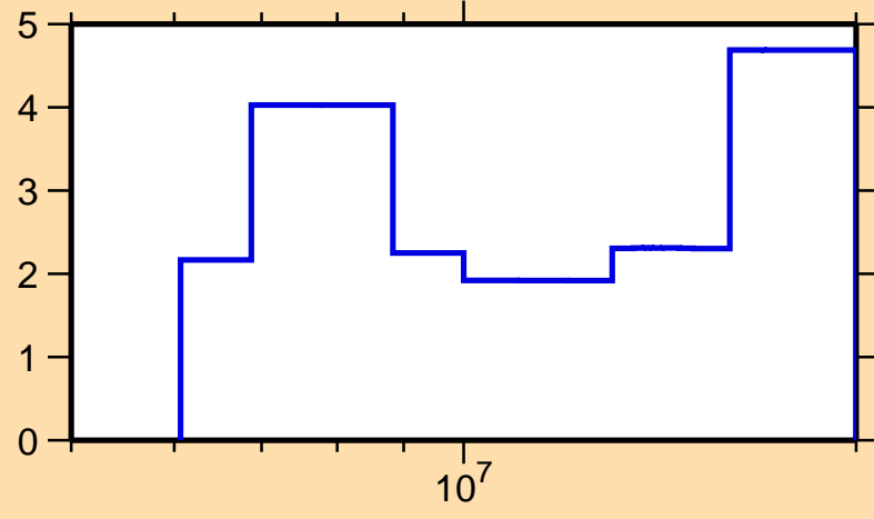
\Delta\sigma/\sigma vs. E for ^{133}\text{Xe}(n,\text{el.})
