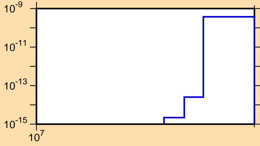
\sigma vs. E for ^{133}\text{Xe}(n,nt)
