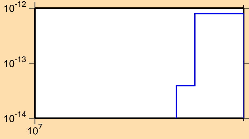
\sigma vs. E for ^{133}\text{Xe}(n,p\alpha)
