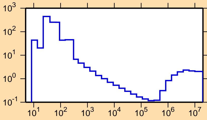
\sigma vs. E for ^{133}\text{Xe}(n,\text{nonel.})
