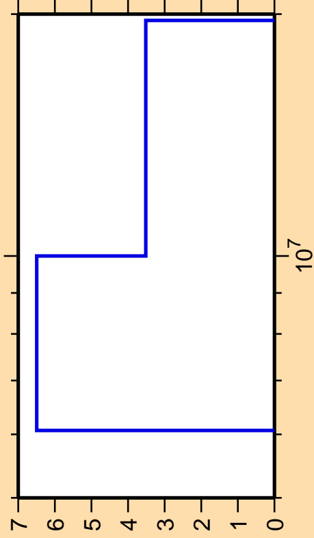
\Delta\sigma/\sigma vs. E for ^{133}\text{Xe}(n,2n)
