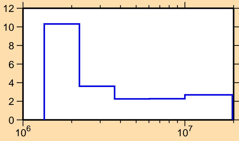
\Delta\sigma/\sigma vs. E for ^{133}\text{Xe}(n,\text{nonel.})
