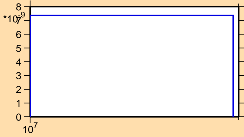
\sigma vs. E for ^{133}\text{Xe}(n,\text{nd})
