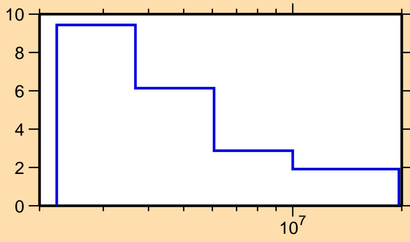
\Delta\sigma/\sigma vs. E for ^{133}\text{Xe}(n,\text{el.})
