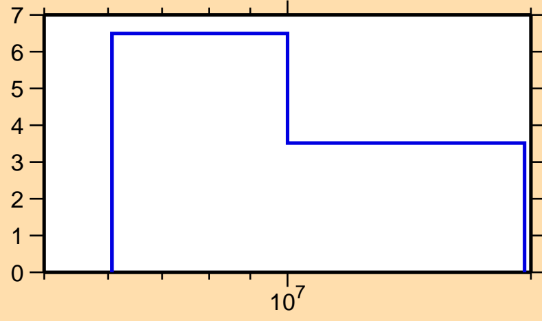
\Delta\sigma/\sigma vs. E for ^{133}\text{Xe}(n,2n)
