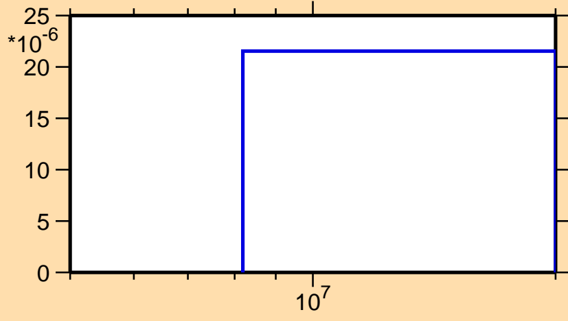
\sigma vs. E for ^{133}\text{Xe}(n,n\alpha)
