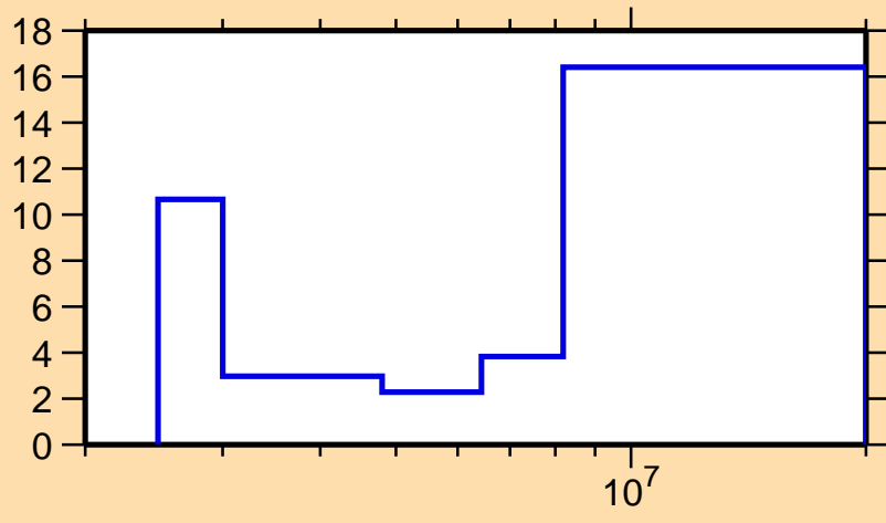
\Delta\sigma/\sigma vs. E for ^{133}\text{Xe}(n,n\text{cont.})
