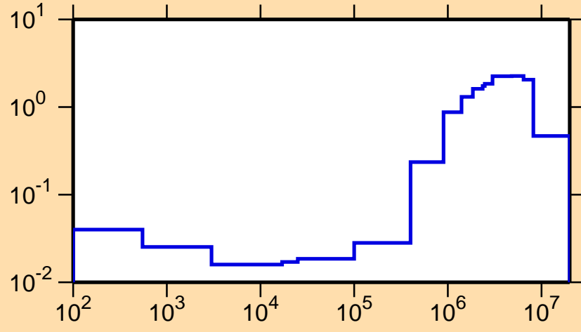
\sigma vs. E for ^{133}\text{Xe}(n,\text{inel.})
