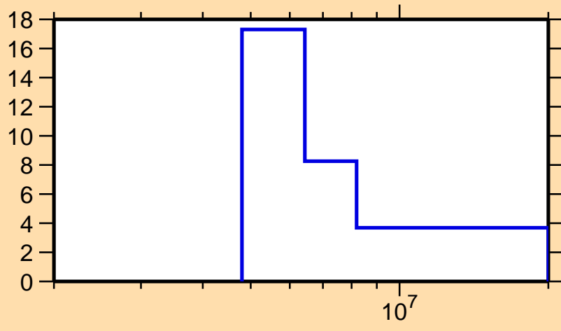
\Delta\sigma/\sigma vs. E for ^{133}\text{Xe}(n,2n)
