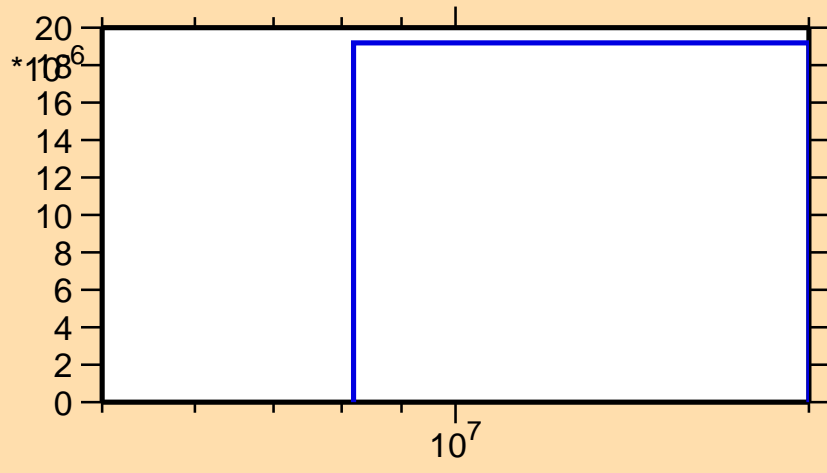
\sigma vs. E for ^{133}\text{Xe}(n,t)
