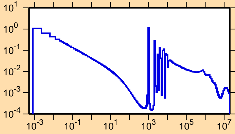
\sigma vs. E for ^{134}\text{Xe}(n,\gamma)
