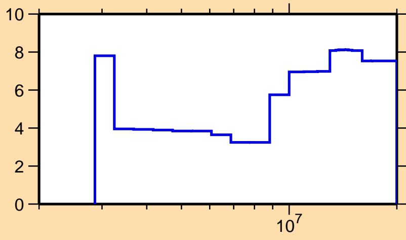
\Delta\sigma/\sigma vs. E for ^{134}\text{Xe}(n,n\text{cont.})
