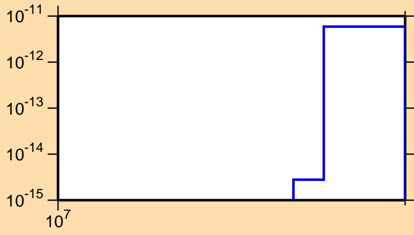
\sigma vs. E for ^{134}\text{Xe}(n,\text{He}3)
