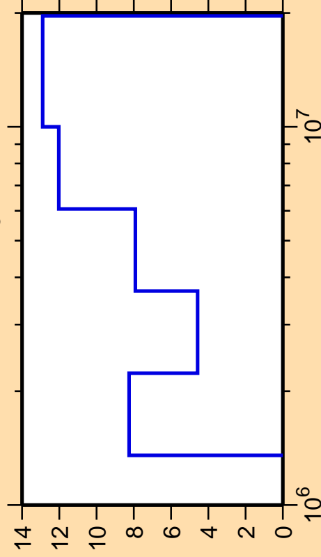
\Delta\sigma/\sigma vs. E for ^{134}\text{Xe}(n,n_3)
