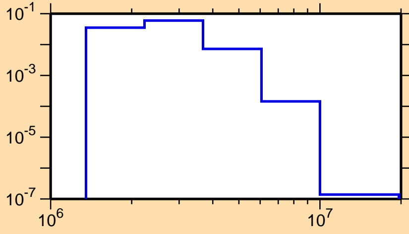
\sigma vs. E for ^{134}\text{Xe}(n,n_3)
