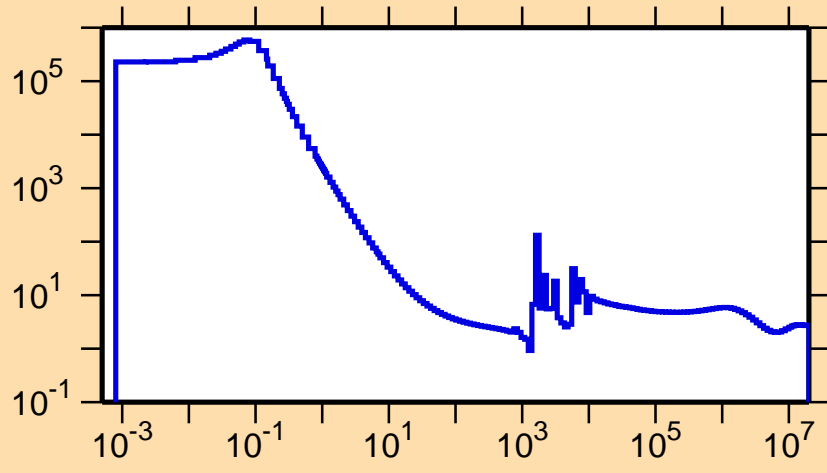
\sigma vs. E for ^{135}\text{Xe}(n,\text{el.})
