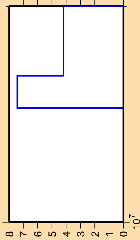
\Delta\sigma/\sigma vs. E for ^{135}\text{Xe}(n,3n)
