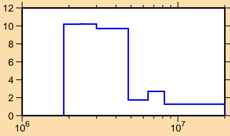
\Delta\sigma/\sigma vs. E for ^{135}\text{Xe}(n, el.)
