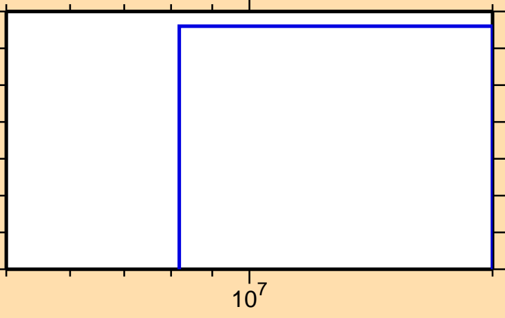
\sigma vs. E for ^{135}\text{Xe}(n,\text{nd})
