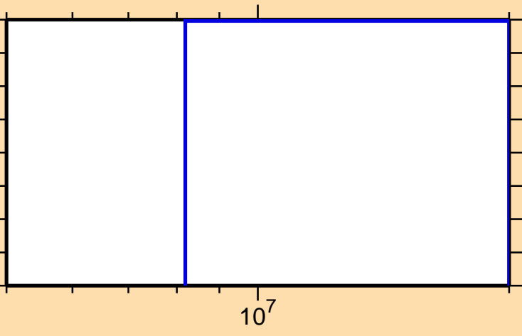
\sigma vs. E for ^{135}\text{Xe}(n,2n\alpha)
