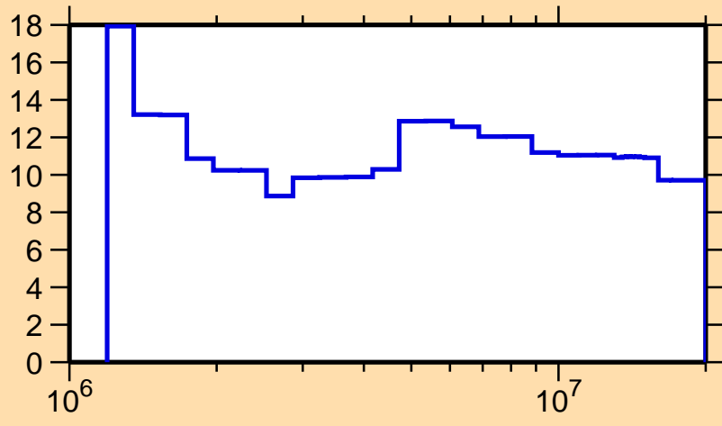
\Delta\sigma/\sigma vs. E for ^{136}\text{Xe}(n,n_1)
