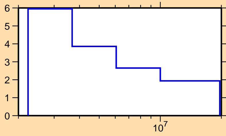
\Delta\sigma/\sigma vs. E for ^{136}\text{Xe}(n,\text{el.})
