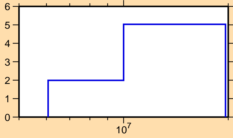
\Delta\sigma/\sigma vs. E for ^{136}\text{Xe}(n,\text{inel.})
