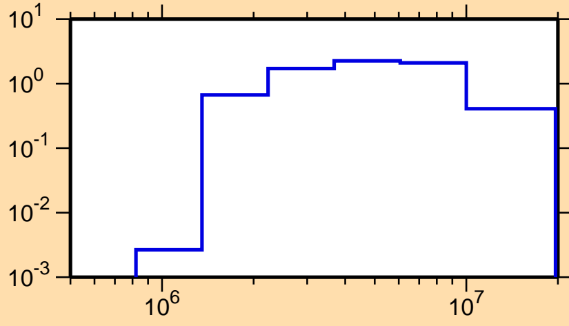
\sigma vs. E for ^{136}\text{Xe}(n,\text{inel.})
