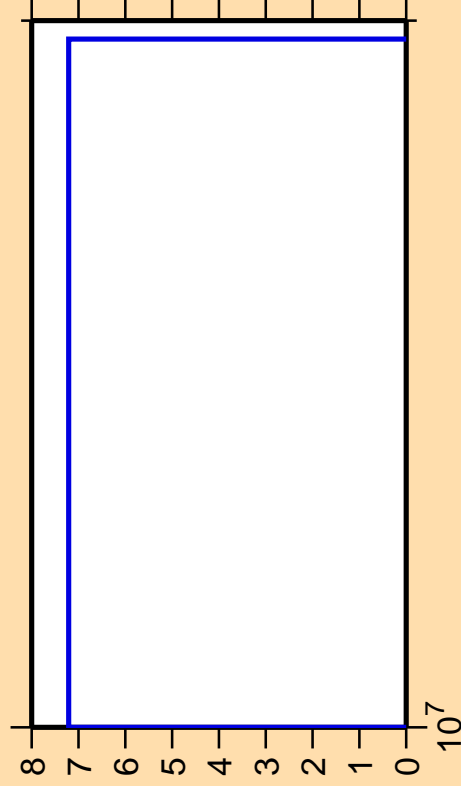
\Delta\sigma/\sigma vs. E for ^{136}\text{Xe}(n,\text{nd})
