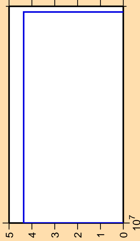
\Delta\sigma/\sigma vs. E for ^{136}\text{Xe}(n,3n)
