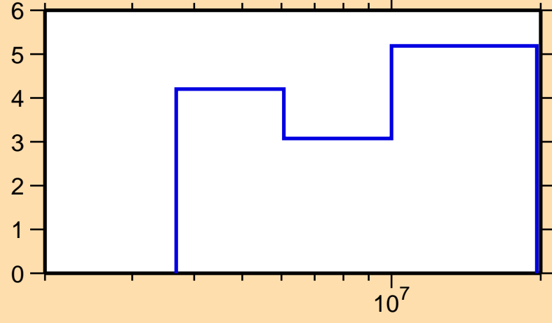
\Delta\sigma/\sigma vs. E for ^{136}\text{Xe}(n,n\text{cont.})
