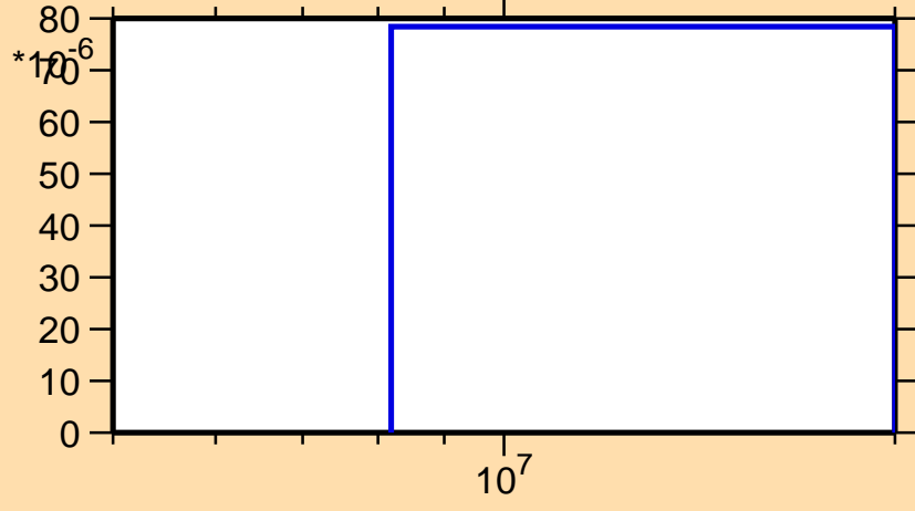
\sigma vs. E for ^{136}\text{Xe}(n,d)
