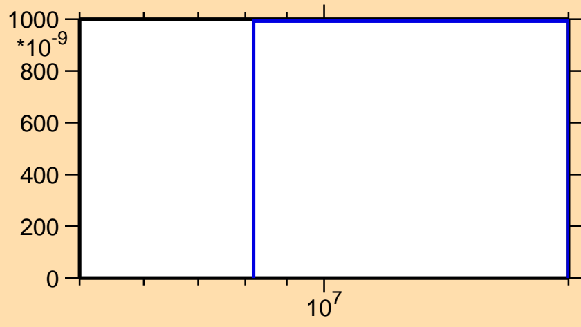
\sigma vs. E for ^{136}\text{Xe}(n,n\alpha)
