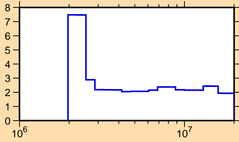
\Delta\sigma/\sigma vs. E for ^{137}\text{Xe}(n,\text{nonel.})
