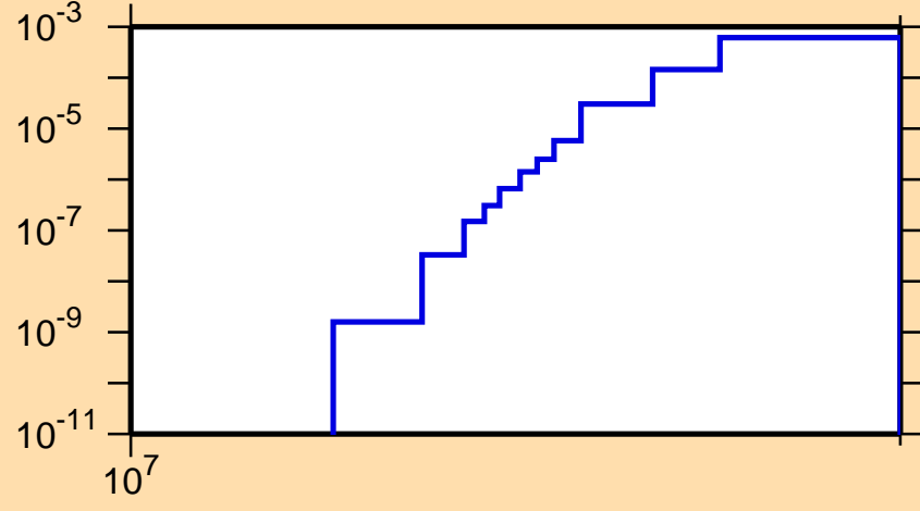
\sigma vs. E for ^{137}\text{Xe}(n,np)
