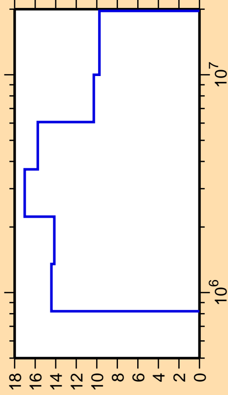
\Delta\sigma/\sigma vs. E for ^{137}\text{Xe}(n,n_4)
