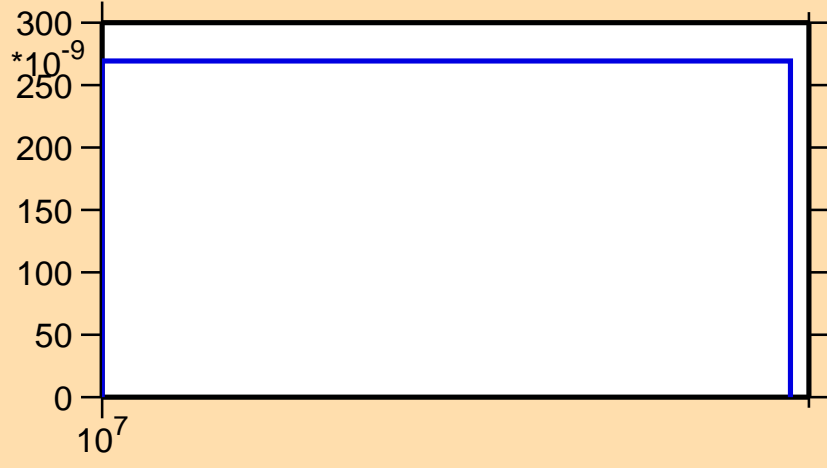
\sigma vs. E for ^{137}\text{Xe}(n,\text{nd})
