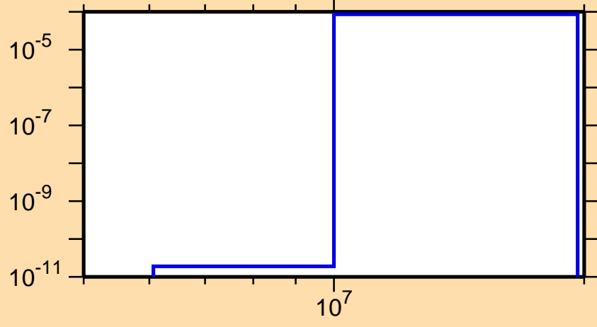
\sigma vs. E for ^{137}\text{Xe}(n,n\alpha)
