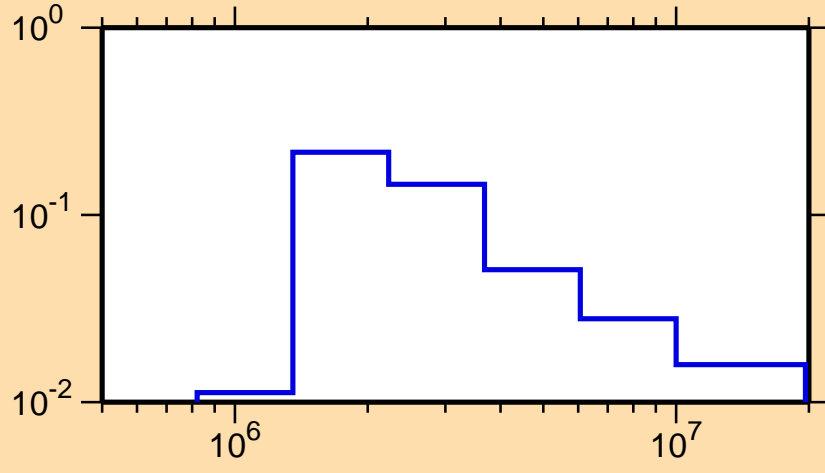
\sigma vs. E for ^{137}\text{Xe}(n,n_4)
