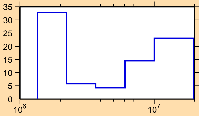
\Delta\sigma/\sigma vs. E for ^{137}\text{Xe}(n,n\text{cont.})
