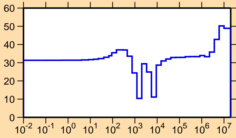
\Delta\sigma/\sigma vs. E for ^{137}\text{Xe}(n,\gamma)
