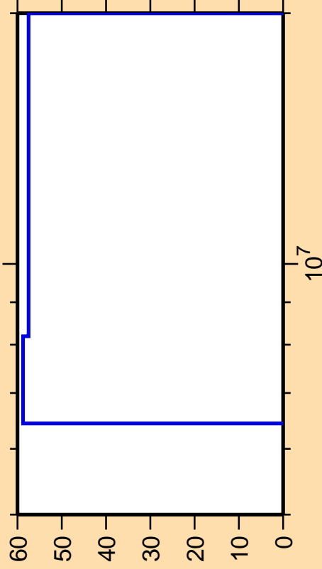
\Delta\sigma/\sigma vs. E for ^{137}\text{Xe}(n,p)
