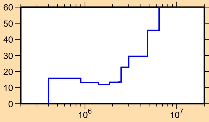
\Delta\sigma/\sigma vs. E for ^{137}\text{Xe}(n,n_1)
