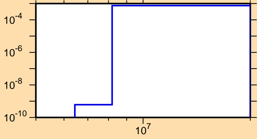
\sigma vs. E for ^{137}\text{Xe}(n,p)
