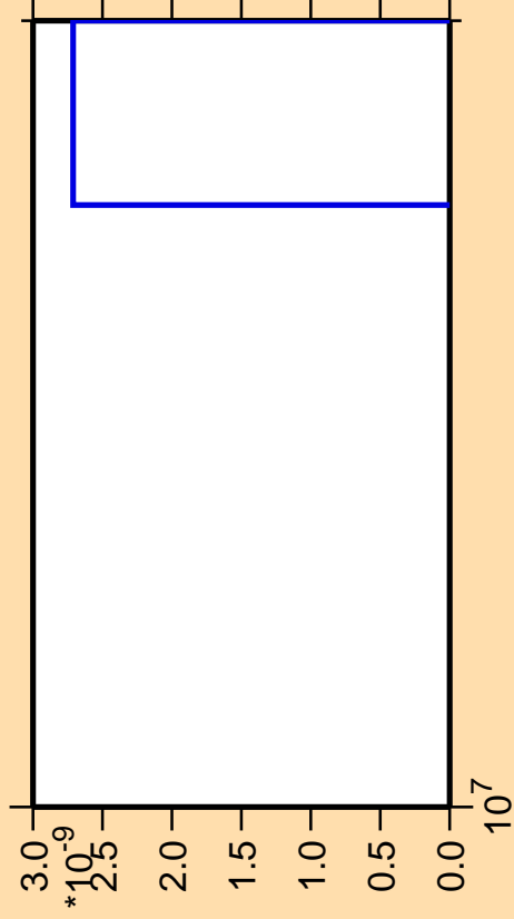
\Delta\sigma/\sigma vs. E for ^{138}\text{Xe} (mt 42)
