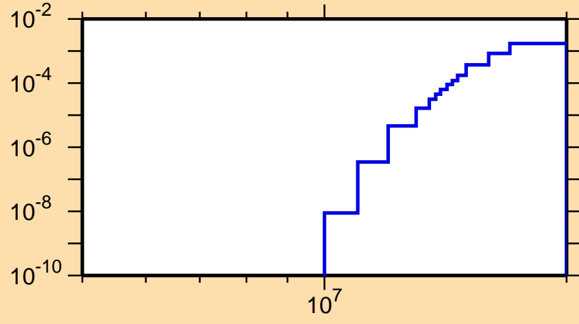
\sigma vs. E for ^{138}\text{Xe}(n,p)
