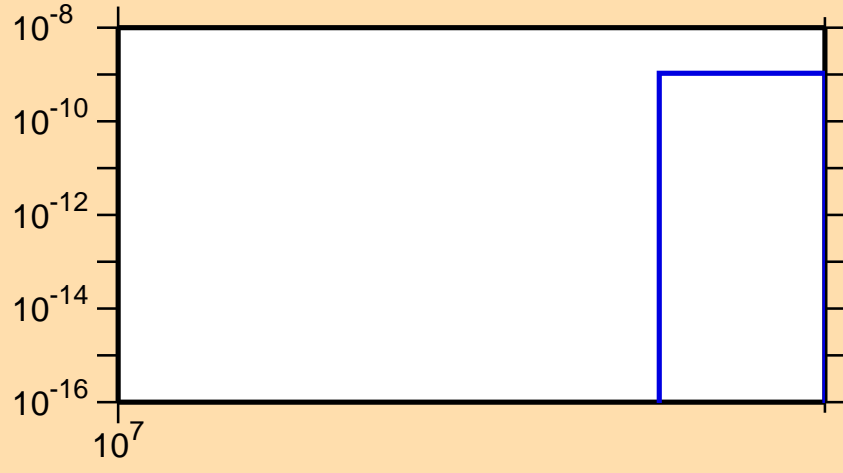
\sigma vs. E for ^{138}\text{Xe}(n,2np)
