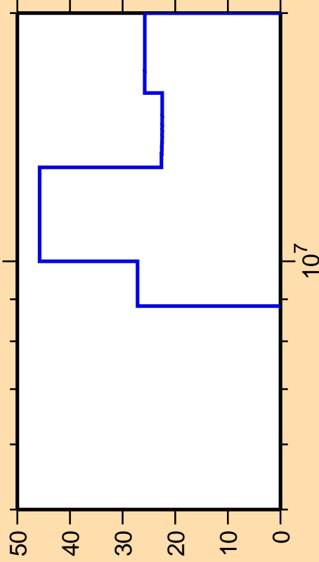
\Delta\sigma/\sigma vs. E for ^{138}\text{Xe}(n,p)
