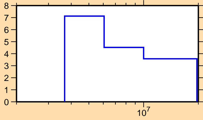
\Delta\sigma/\sigma vs. E for ^{138}\text{Xe}(n,\text{el.})
