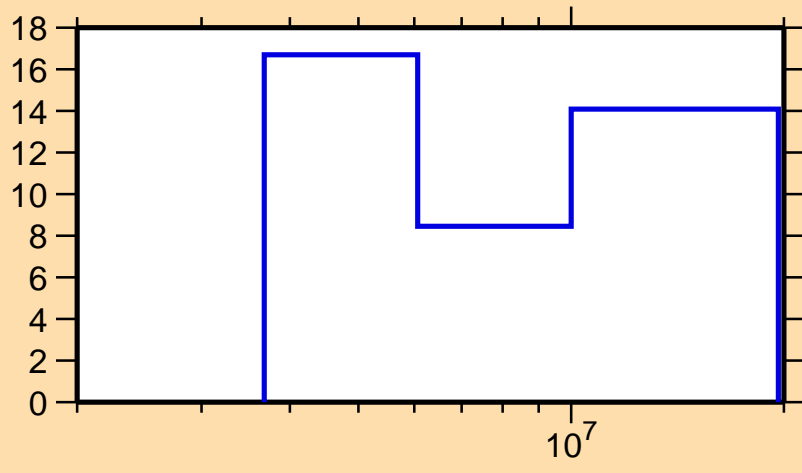
\Delta\sigma/\sigma vs. E for ^{138}\text{Xe}(n,2n)
