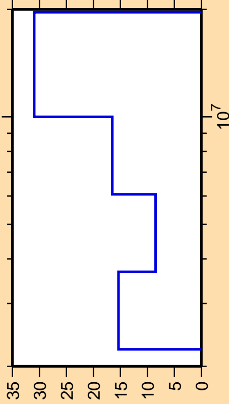
\Delta\sigma/\sigma vs. E for ^{138}\text{Xe}(n,n\text{cont.})
