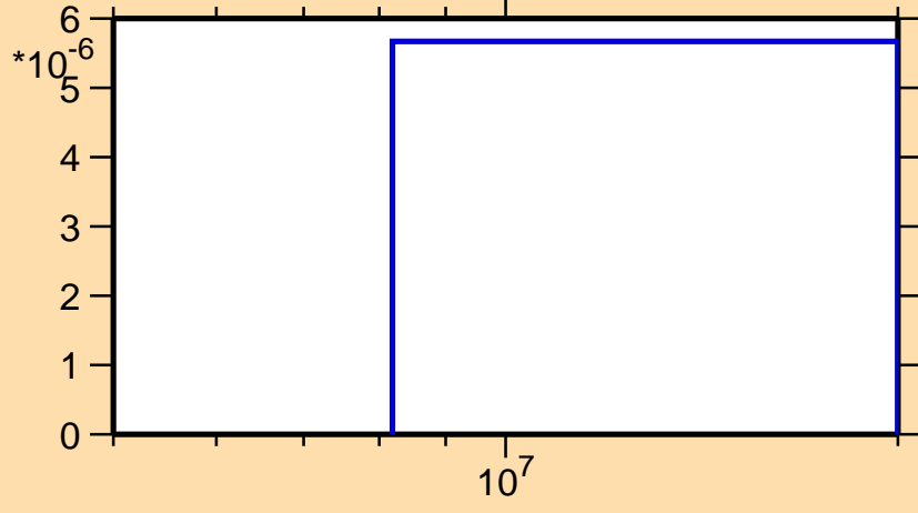
\sigma vs. E for ^{138}\text{Xe}(n,np)
