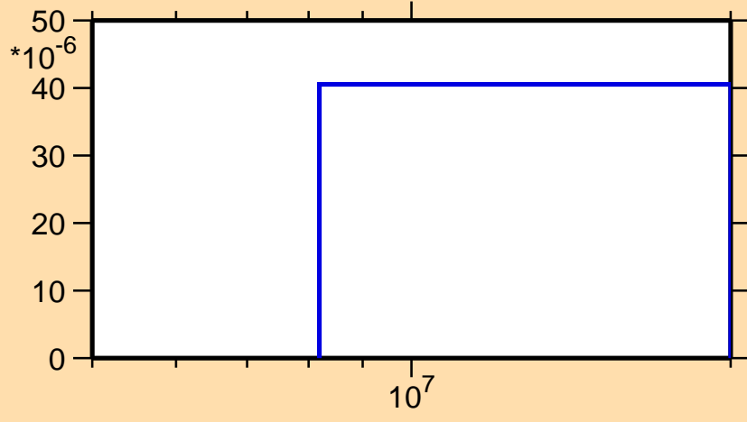
\sigma vs. E for ^{138}\text{Xe}(n,t)
