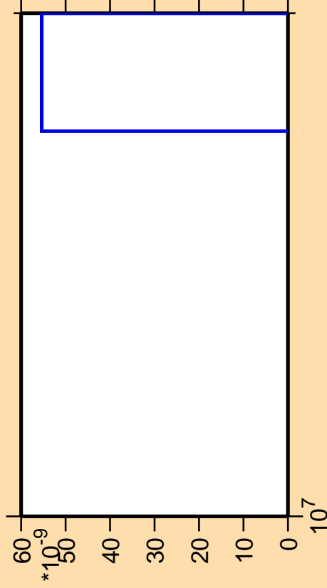
\Delta\sigma/\sigma vs. E for ^{139}\text{Xe} (mt 42)
