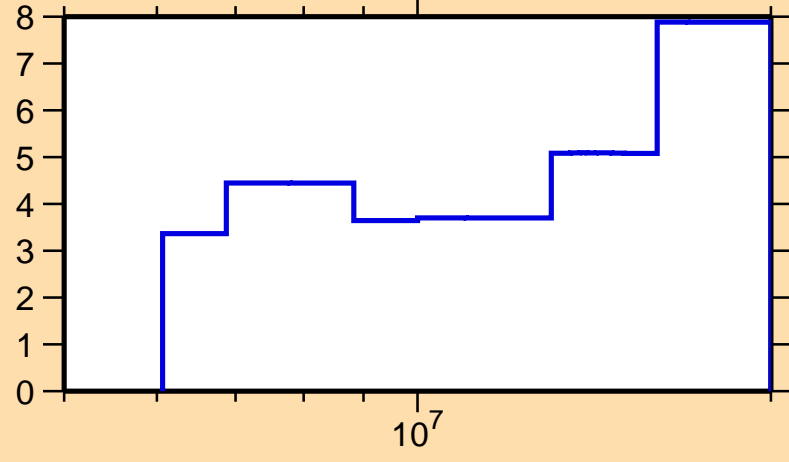
\Delta\sigma/\sigma vs. E for ^{139}\text{Xe}(n,\text{el.})
