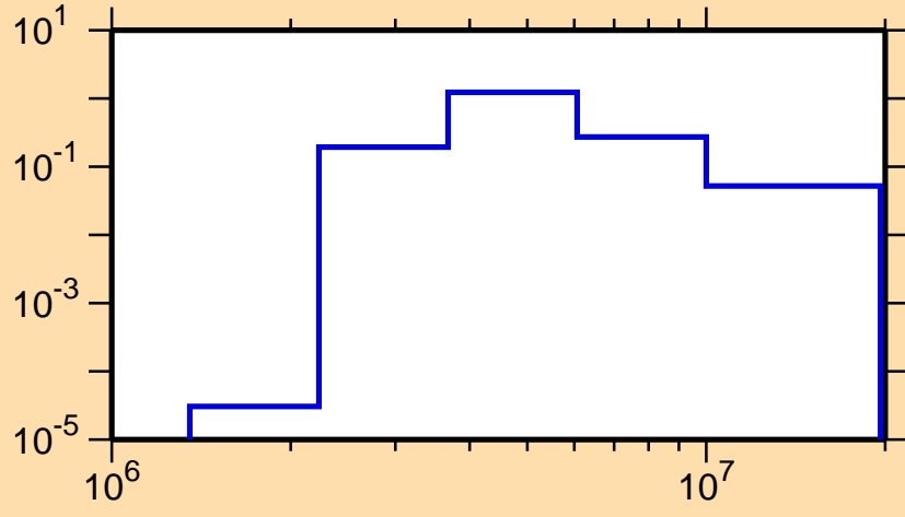
\sigma vs. E for ^{139}\text{Xe}(n,n\text{cont.})
