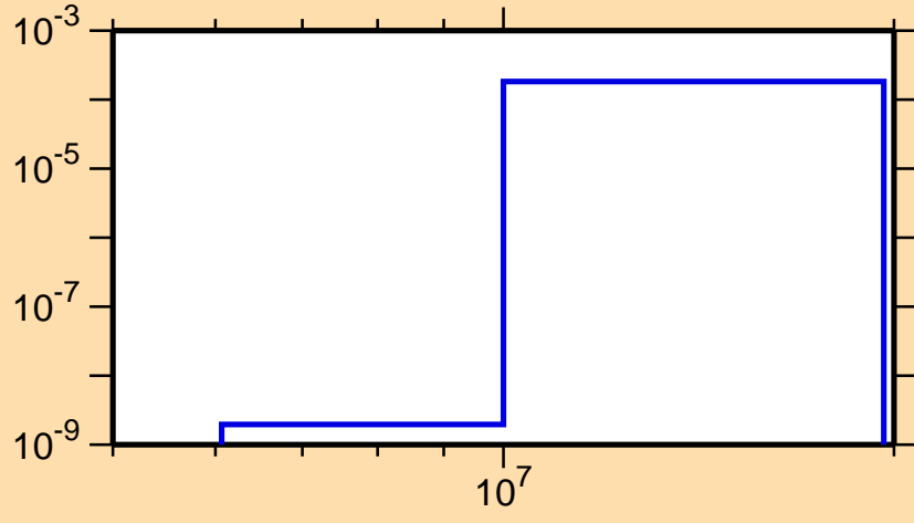
\sigma vs. E for ^{139}\text{Xe}(n,n\alpha)
