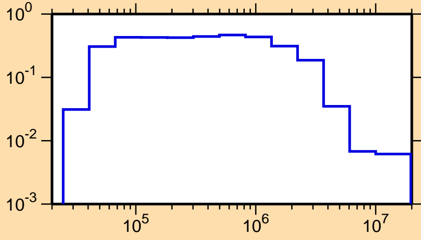
\sigma vs. E for ^{139}\text{Xe}(n,n_2)
