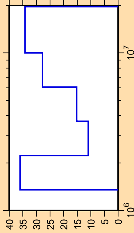
\Delta\sigma/\sigma vs. E for ^{139}\text{Xe}(n,n\text{cont.})
