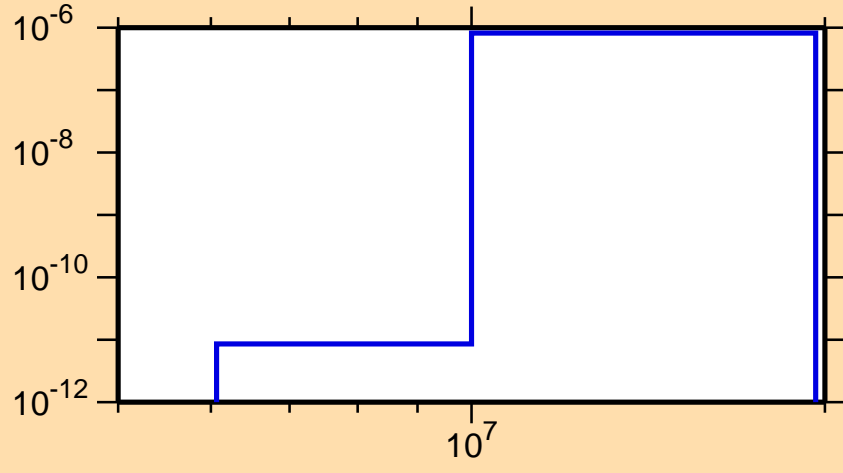
\sigma vs. E for ^{139}\text{Xe}(n,2n\alpha)
