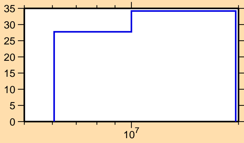
\Delta\sigma/\sigma vs. E for ^{139}\text{Xe}(n,n\text{cont.})
