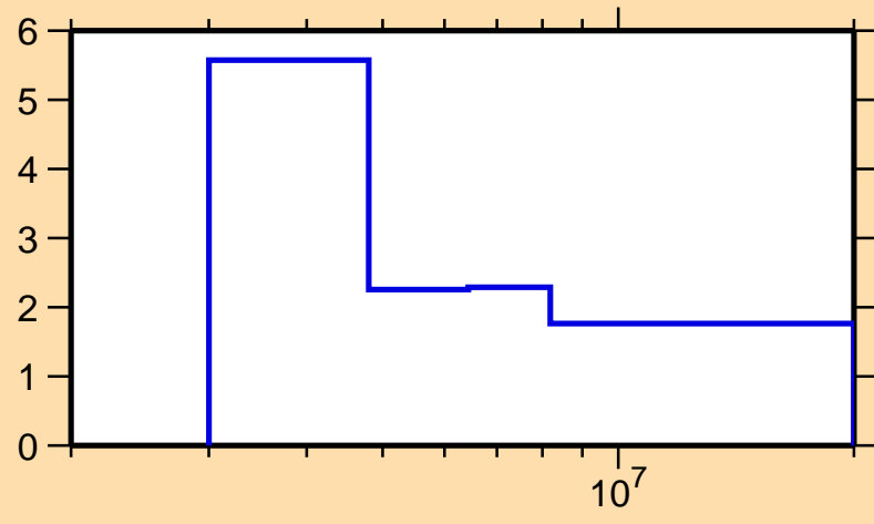
\Delta\sigma/\sigma vs. E for ^{139}\text{Xe}(n,\text{tot.})
