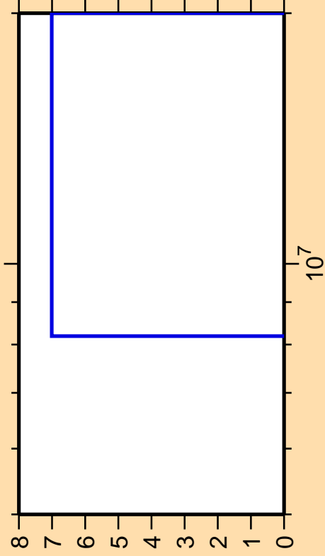
\Delta\sigma/\sigma vs. E for ^{139}\text{Xe}(n,3n)
