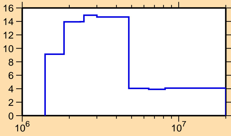
\Delta\sigma/\sigma vs. E for ^{139}\text{Xe}(n, el.)
