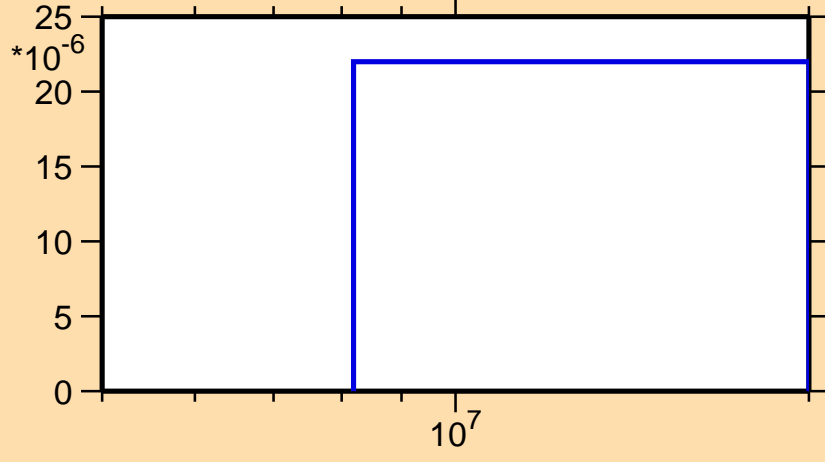
\sigma vs. E for ^{139}\text{Xe}(n,d)
