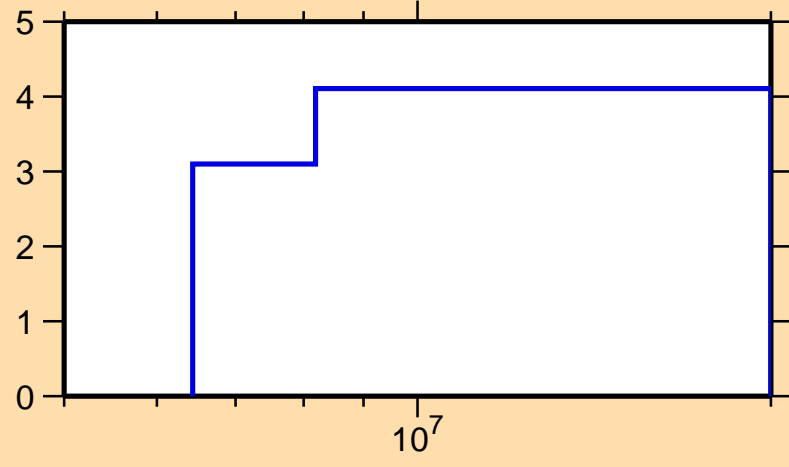
\Delta\sigma/\sigma vs. E for ^{139}\text{Xe}(n,\text{nonel.})
