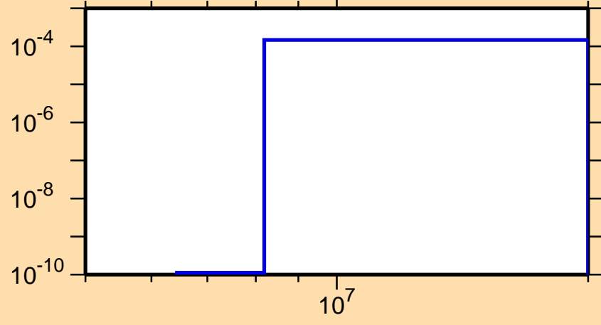
\sigma vs. E for ^{139}\text{Xe}(n,n\alpha)
