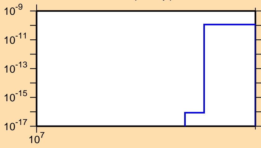
\sigma vs. E for ^{140}\text{Xe}(n,2np)
