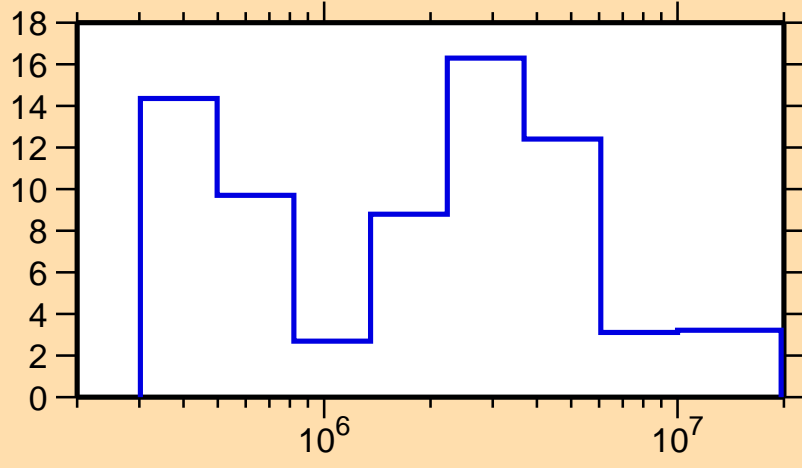
\Delta\sigma/\sigma vs. E for ^{140}\text{Xe}(n,\text{el.})
