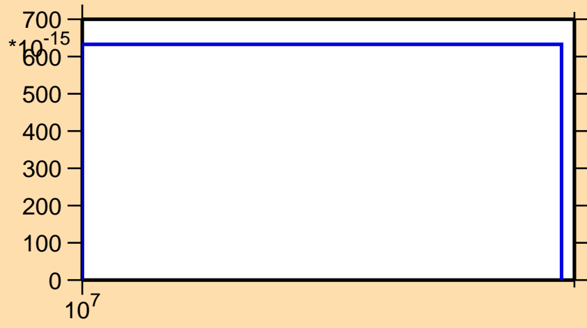
\sigma vs. E for ^{140}\text{Xe}(n,2np)
