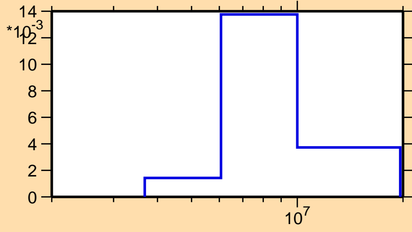
\sigma vs. E for ^{140}\text{Xe}(n,n\text{cont.})
