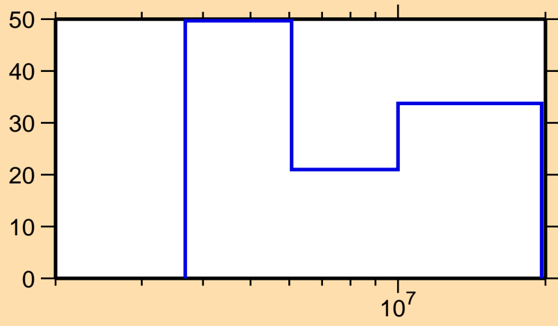
\Delta\sigma/\sigma vs. E for ^{140}\text{Xe}(n,n\text{cont.})
