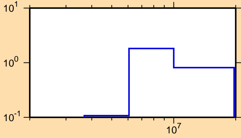
\sigma vs. E for ^{140}\text{Xe}(n,2n)
