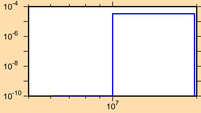
\sigma vs. E for ^{140}\text{Xe}(n,n\alpha)
