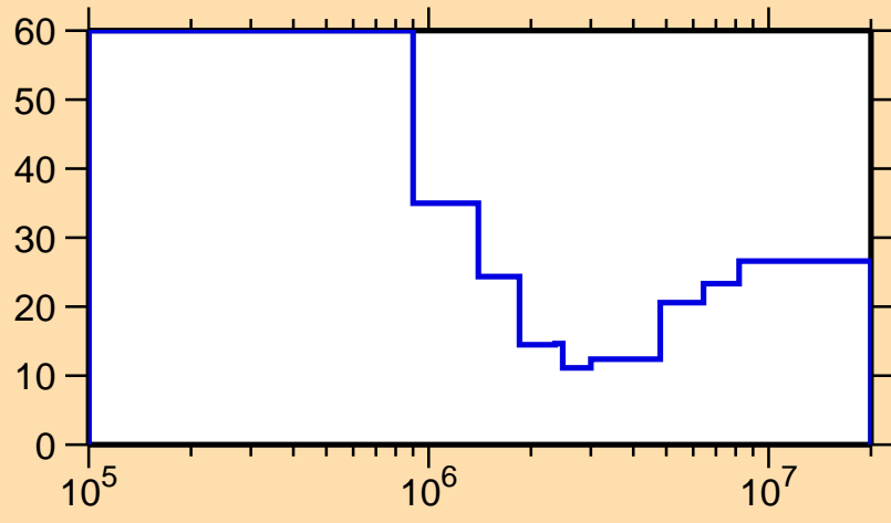
\Delta\sigma/\sigma vs. E for ^{140}\text{Xe}(n,n_1)
