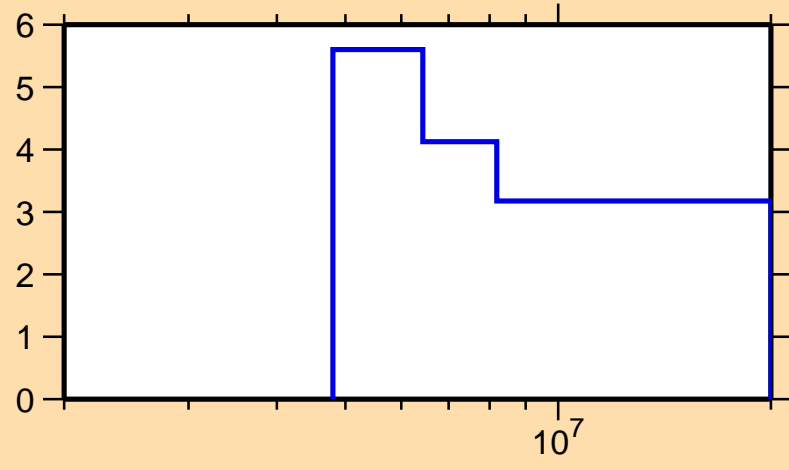
\Delta\sigma/\sigma vs. E for ^{140}\text{Xe}(n,\text{tot.})
