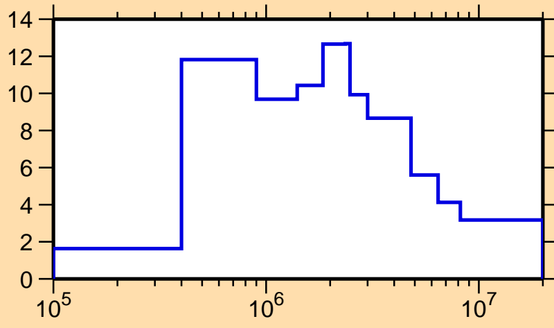
\Delta\sigma/\sigma vs. E for ^{140}\text{Xe}(n,\text{tot.})
