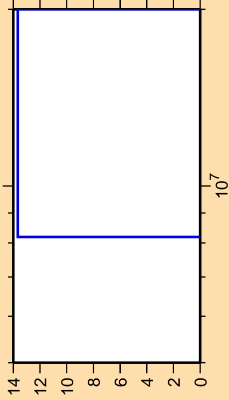
\Delta\sigma/\sigma vs. E for ^{140}\text{Xe}(n,3n)
