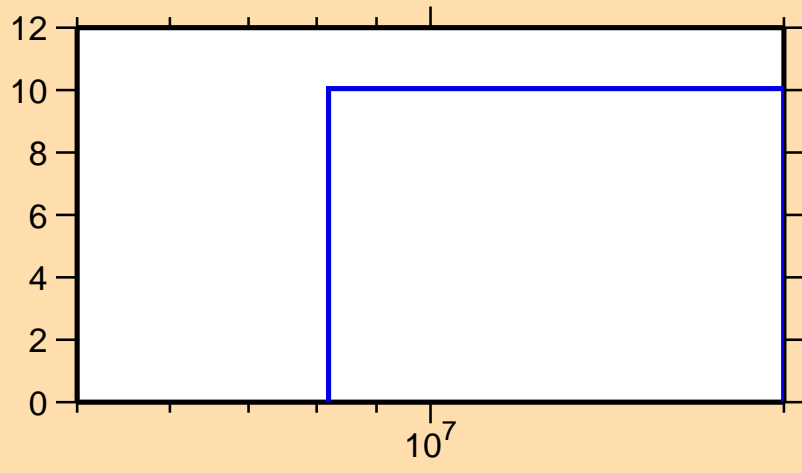
\Delta\sigma/\sigma vs. E for ^{140}\text{Xe}(n,\text{nonel.})
