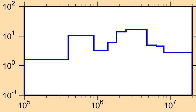
\Delta\sigma/\sigma vs. E for ^{140}\text{Xe}(n,\text{el.})
