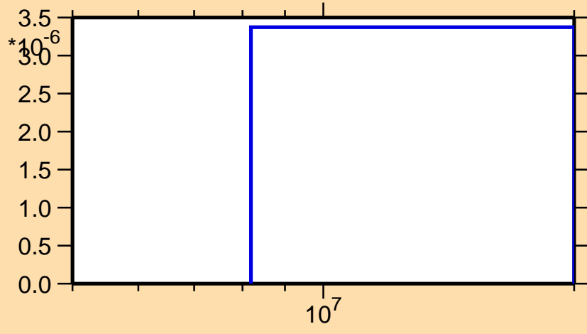
\sigma vs. E for ^{140}\text{Xe}(n,d)
