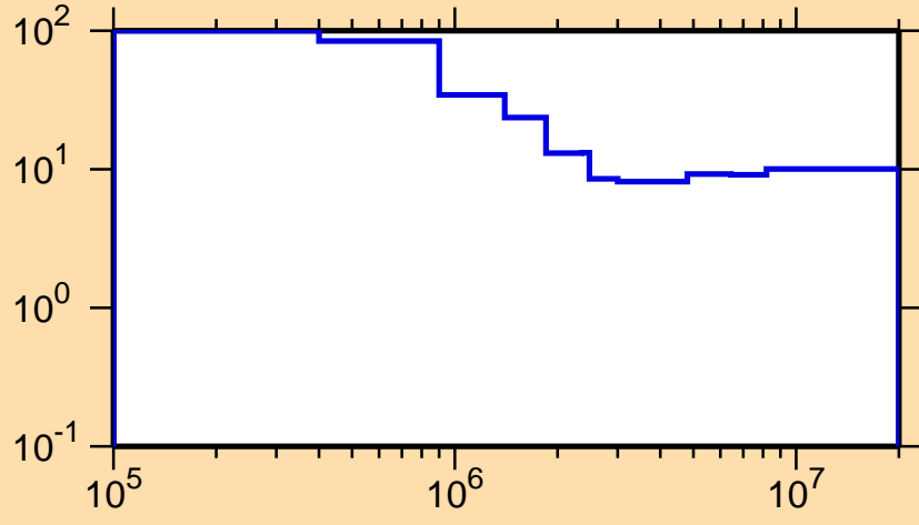
\Delta\sigma/\sigma vs. E for ^{140}\text{Xe}(n,\text{nonel.})
