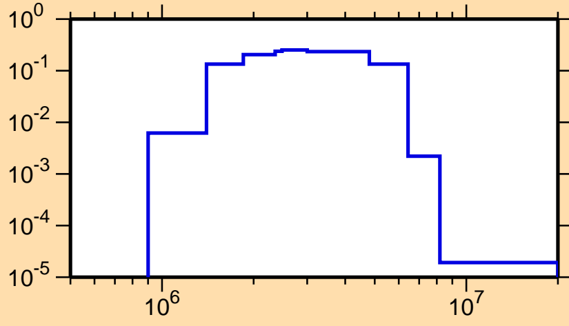
\sigma vs. E for ^{140}\text{Xe}(n,n_3)
