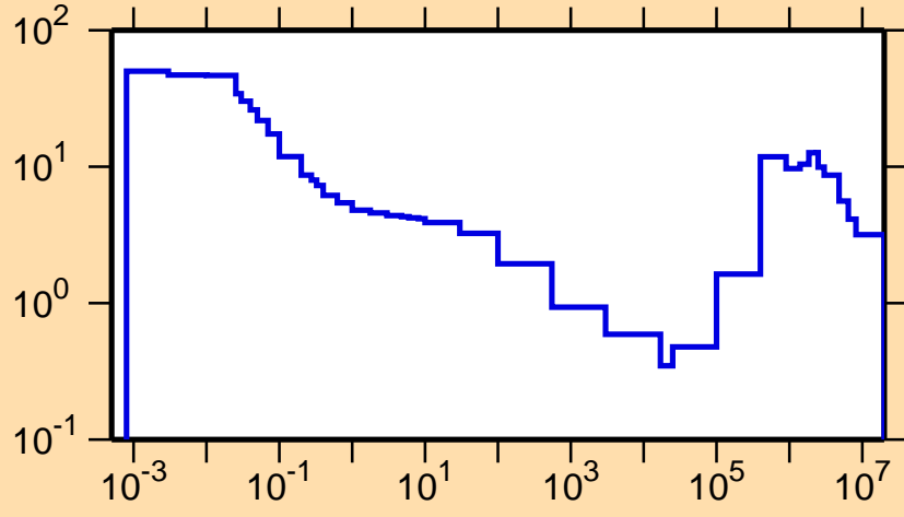
\Delta\sigma/\sigma vs. E for ^{140}\text{Xe}(n,\text{tot.})
