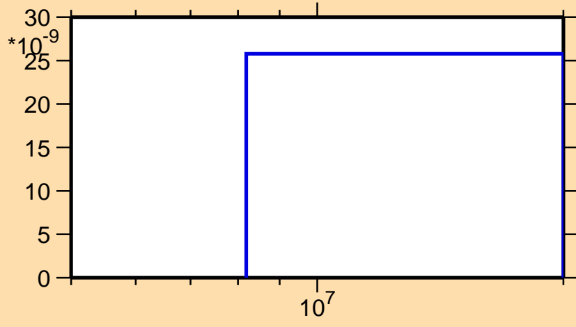
\sigma vs. E for ^{140}\text{Xe}(n,2n\alpha)
