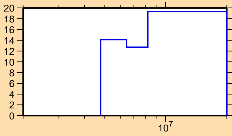
\Delta\sigma/\sigma vs. E for ^{140}\text{Xe}(n,2n)
