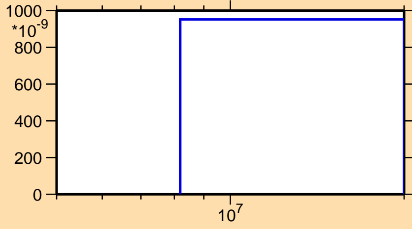
\sigma vs. E for ^{140}\text{Xe}(n,np)
