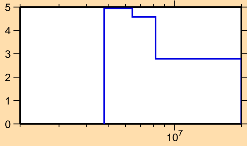
\Delta\sigma/\sigma vs. E for ^{140}\text{Xe}(n,\text{el.})
