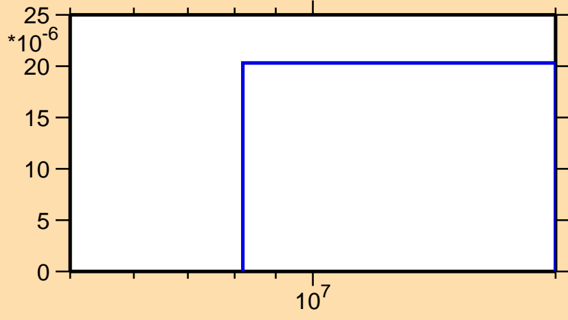
\sigma vs. E for ^{140}\text{Xe}(n,p)
