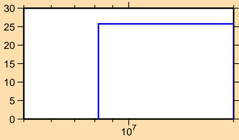
\Delta\sigma/\sigma vs. E for ^{140}\text{Xe}(n,\text{inel.})
