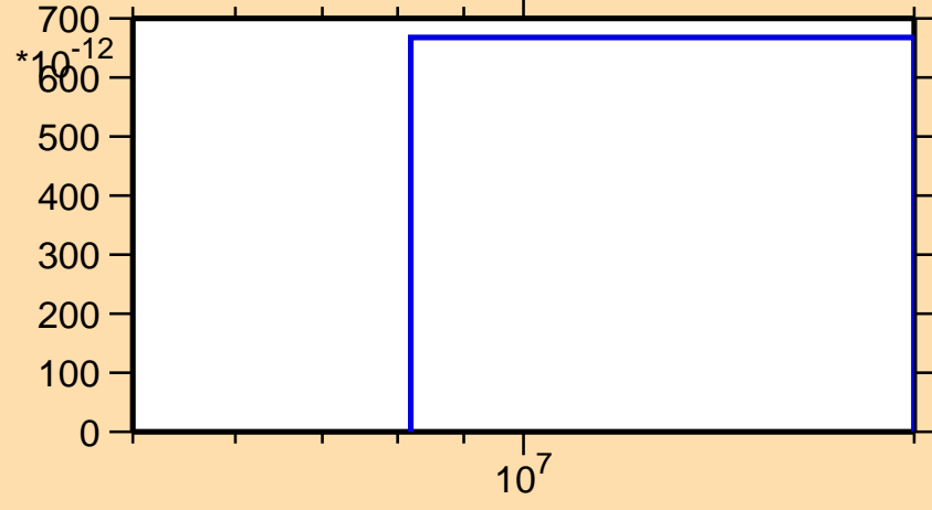
\sigma vs. E for ^{140}\text{Xe}(n,\text{nd})
