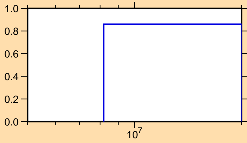
\sigma vs. E for ^{140}\text{Xe}(n,3n)
