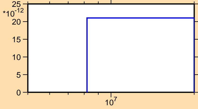
\sigma vs. E for ^{140}\text{Xe}(n,3n\alpha)
