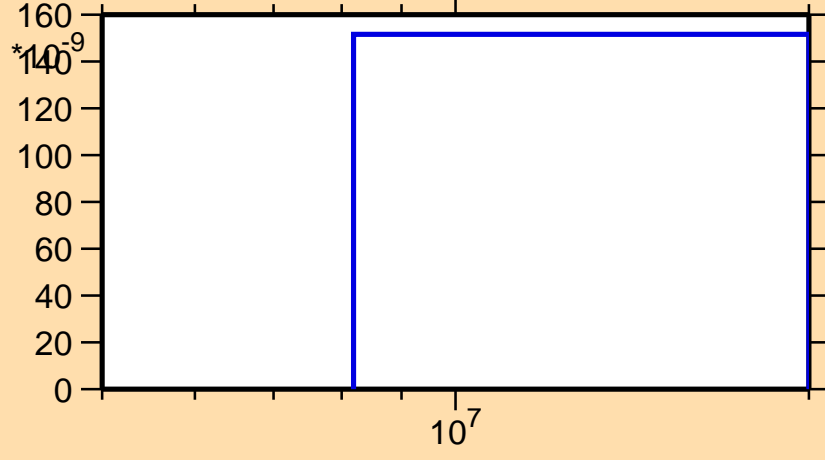
\sigma vs. E for ^{140}\text{Xe}(n,nt)
