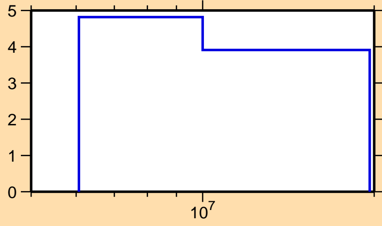
\Delta\sigma/\sigma vs. E for ^{141}\text{Xe}(n,\text{tot.})
