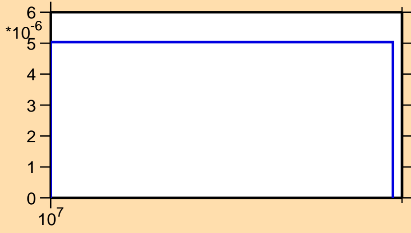
\sigma vs. E for ^{141}\text{Xe}(n,d)
