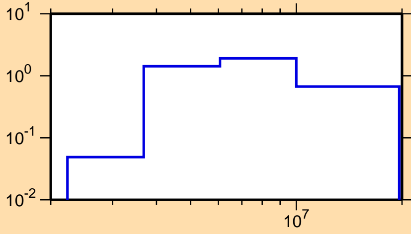
\sigma vs. E for ^{141}\text{Xe}(n,2n)
