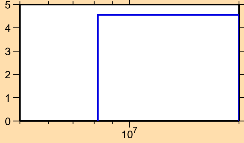
\Delta\sigma/\sigma vs. E for ^{141}\text{Xe}(n,el.)
