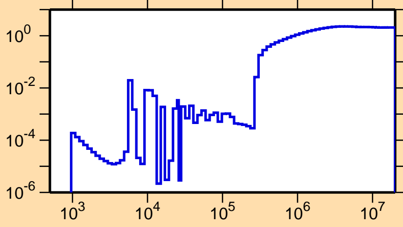
\sigma vs. E for ^{142}\text{Xe}(n,\text{nonel.})
