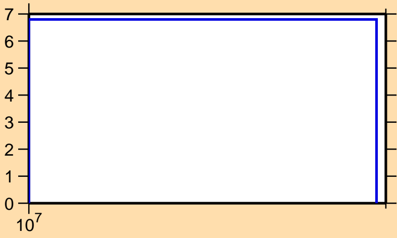
\Delta\sigma/\sigma vs. E for ^{142}\text{Xe}(n,el.)
