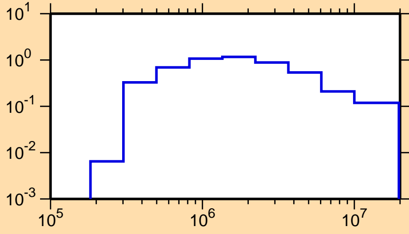
\sigma vs. E for ^{142}\text{Xe}(n,n_1)
