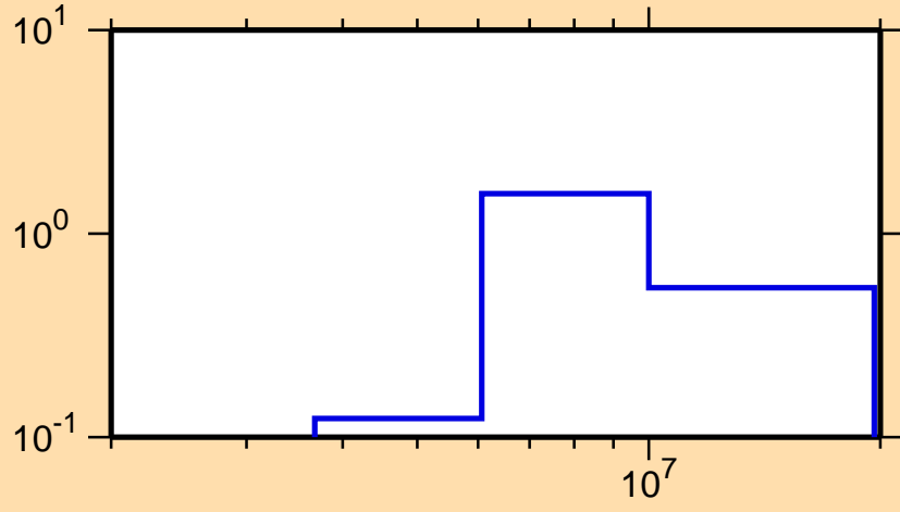
\sigma vs. E for ^{142}\text{Xe}(n,2n)
