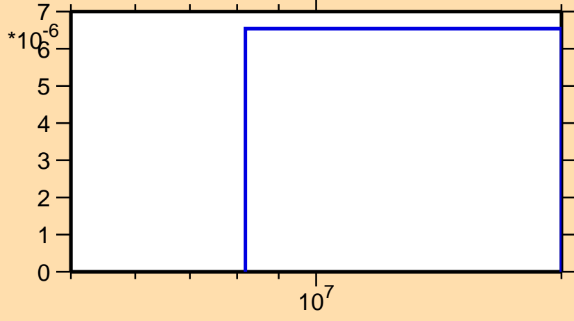
\sigma vs. E for ^{142}\text{Xe}(n,n\alpha)
