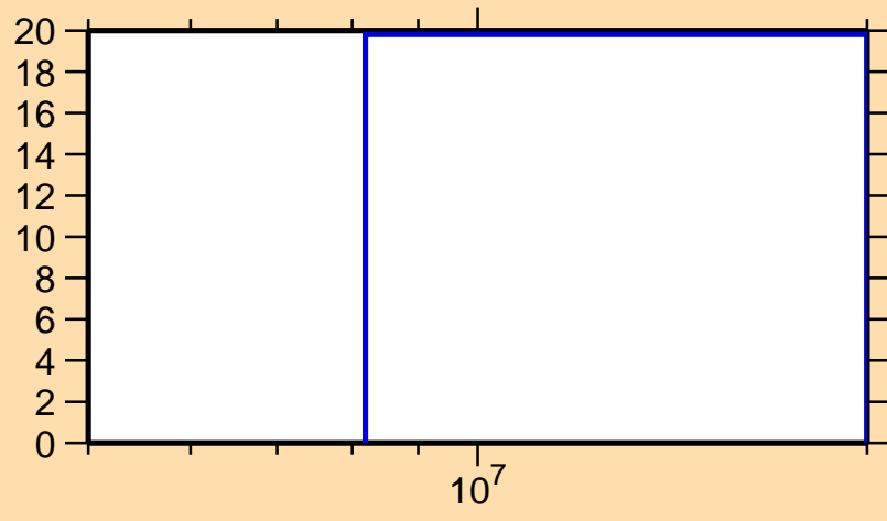
\Delta\sigma/\sigma vs. E for ^{142}\text{Xe}(n,\text{inel.})
