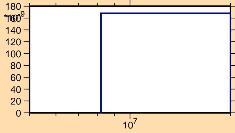
\sigma vs. E for ^{142}\text{Xe}(n,np)
