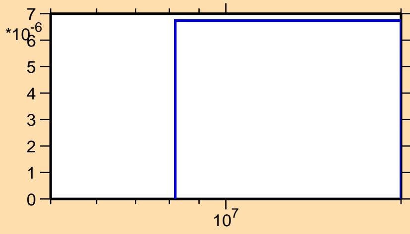
\sigma vs. E for ^{142}\text{Xe}(n,t)
