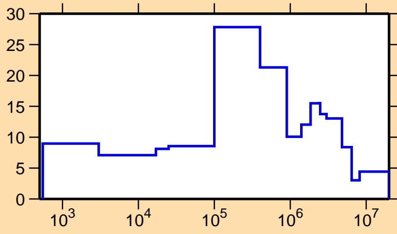
\Delta\sigma/\sigma vs. E for ^{142}\text{Xe}(n,\text{tot.})
