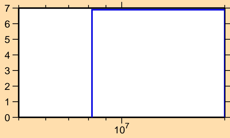
\Delta\sigma/\sigma vs. E for ^{142}\text{Xe}(n,\text{nonel.})
