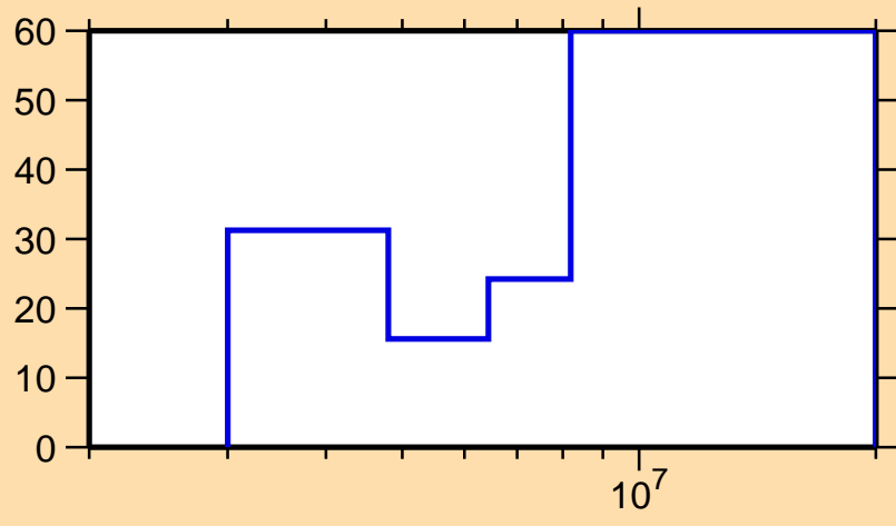
\Delta\sigma/\sigma vs. E for ^{142}\text{Xe}(n,n\text{cont.})
