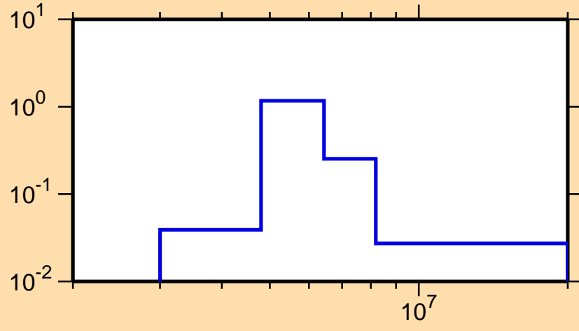
\sigma vs. E for ^{142}\text{Xe}(n,n\text{cont.})
