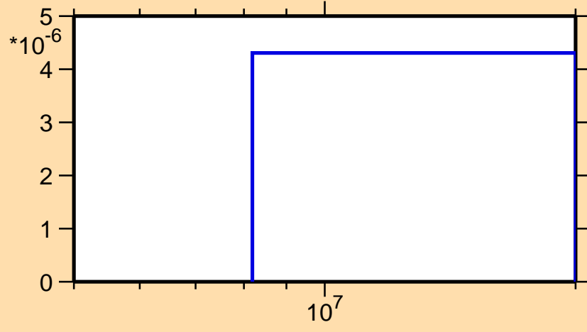
\sigma vs. E for ^{142}\text{Xe}(n,p)
