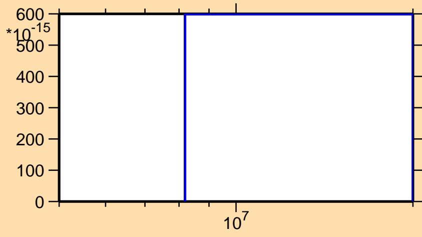
\sigma vs. E for ^{142}\text{Xe}(n,3n\alpha)
