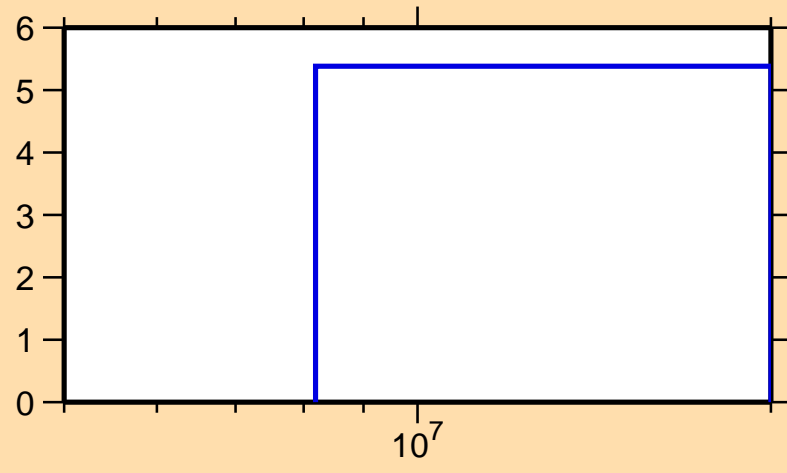
\Delta\sigma/\sigma vs. E for ^{142}\text{Xe}(n,\text{el.})
