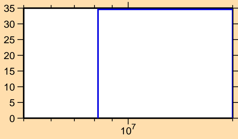
\Delta\sigma/\sigma vs. E for ^{142}\text{Xe}(n,2n)
