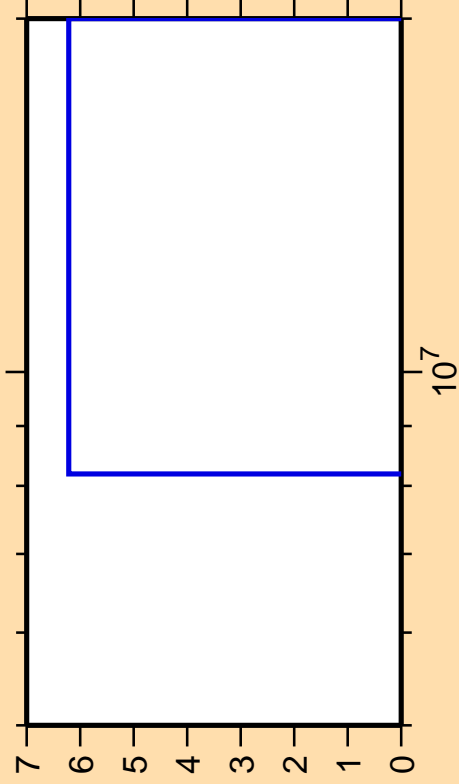
\Delta\sigma/\sigma vs. E for ^{142}\text{Xe}(n,3n)
