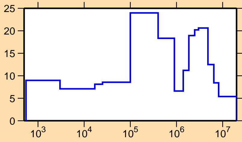
\Delta\sigma/\sigma vs. E for ^{142}\text{Xe}(n,\text{el.})
