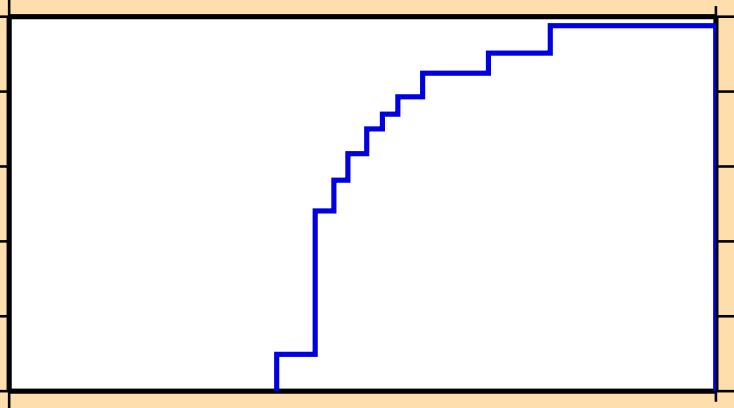
\sigma vs. E for ^{78}\text{Y}(n,2n)
