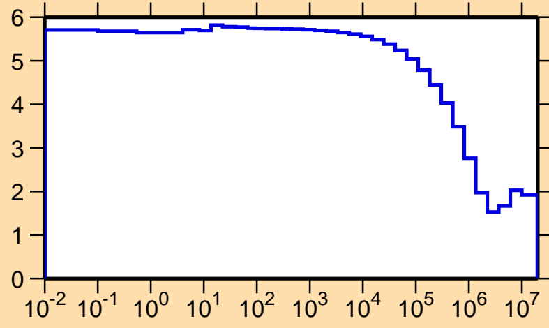
\sigma vs. E for ^{78}\text{Y}(n,\text{el.})
