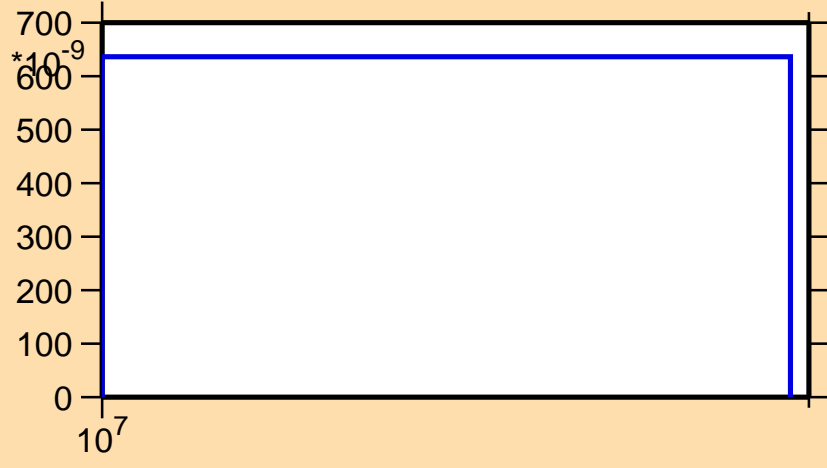
\sigma vs. E for ^{78}\text{Y}(n,2n)
