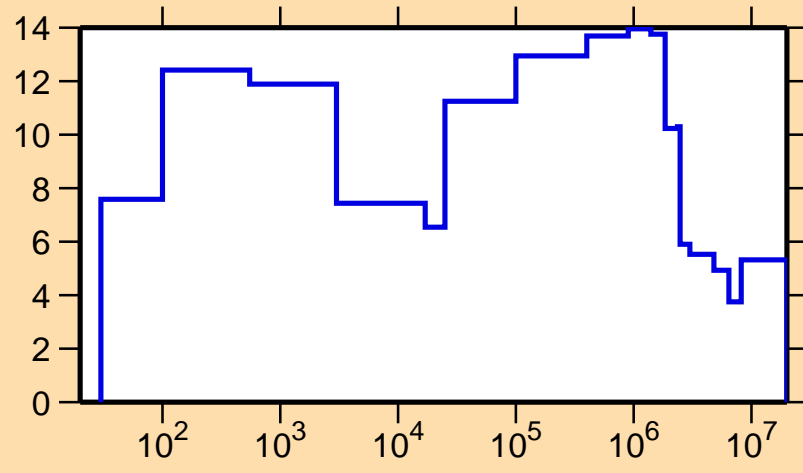
\Delta\sigma/\sigma vs. E for ^{78}\text{Y}(n,\text{tot.})
