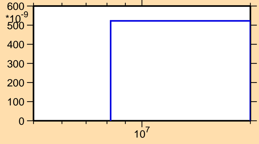
\sigma vs. E for ^{78}\text{Y}(n,2n)
