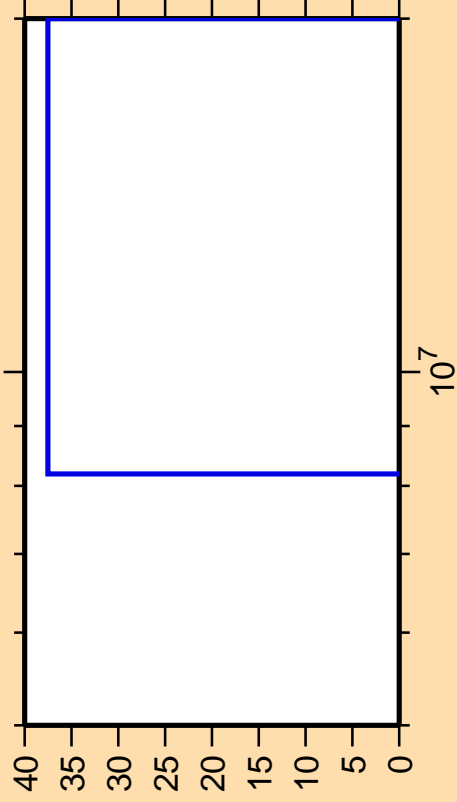
\Delta\sigma/\sigma vs. E for ^{78}\text{Y}(n,p)
