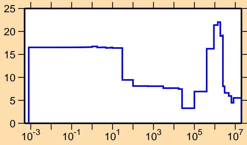
\Delta\sigma/\sigma vs. E for ^{78}\text{Y}(n,\text{el.})
