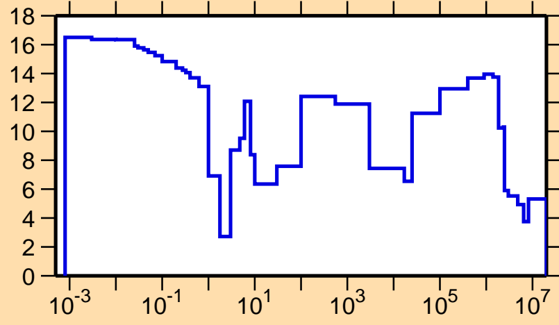
\Delta\sigma/\sigma vs. E for ^{78}\text{Y}(n,\text{tot.})
