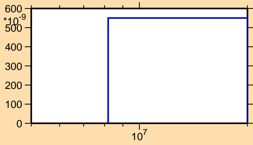
\sigma vs. E for ^{78}\text{Y} (mt 45)
