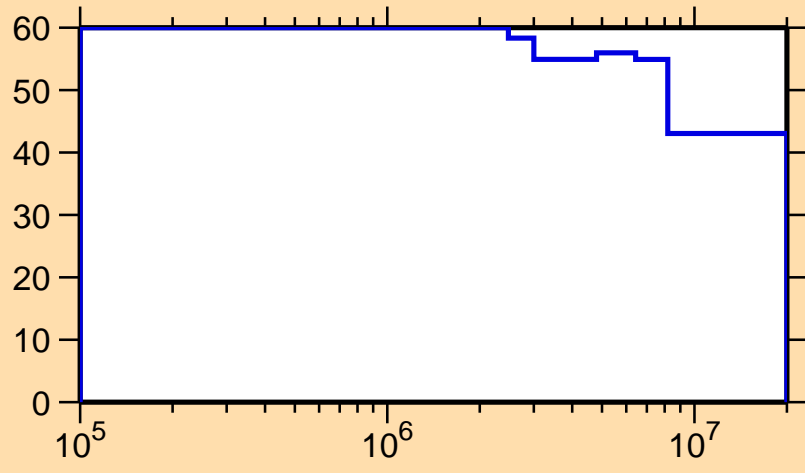
\Delta\sigma/\sigma vs. E for ^{78}\text{Y}(n,n\text{cont.})
