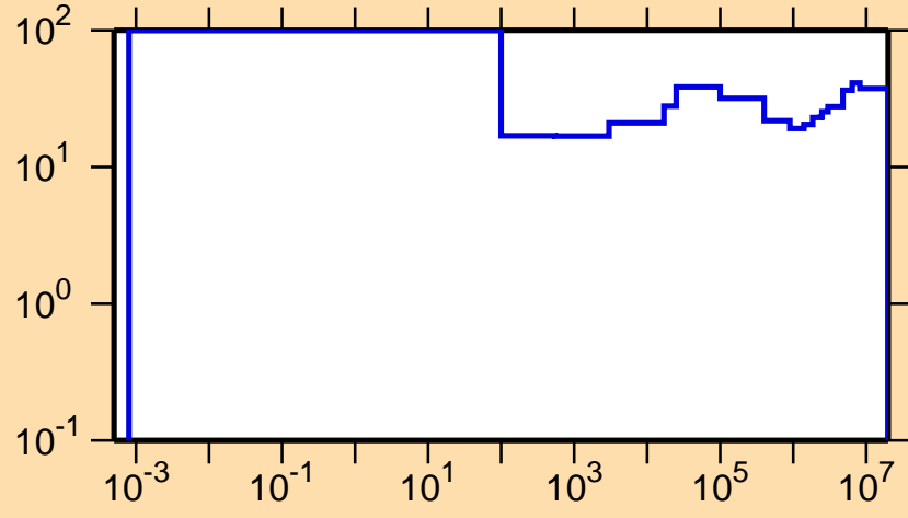
\Delta\sigma/\sigma vs. E for ^{78}\text{Y}(n,p)
