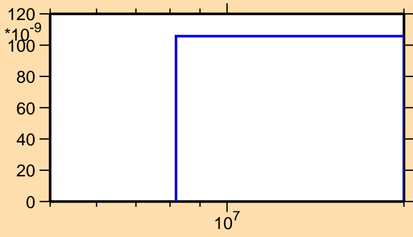
\sigma vs. E for ^{78}\text{Y}(n,nd)
