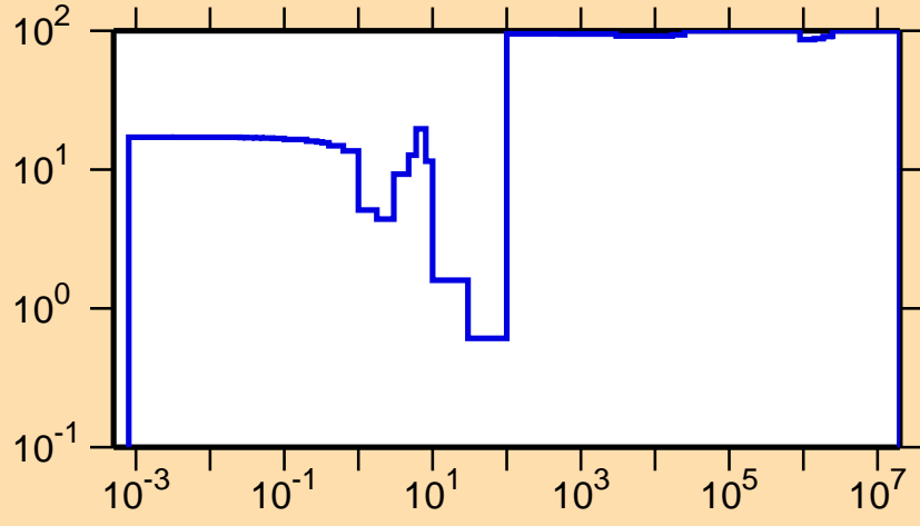
\Delta\sigma/\sigma vs. E for ^{78}\text{Y}(n,\gamma)
