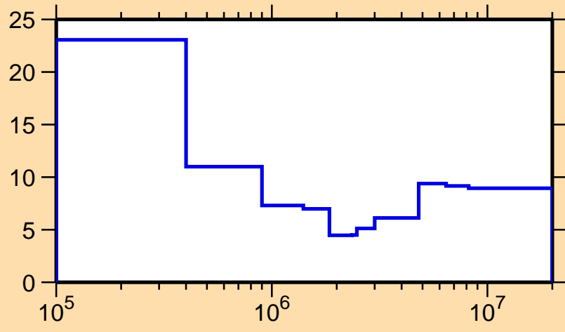
\Delta\sigma/\sigma vs. E for ^{78}\text{Y}(n,n\text{onel.})
