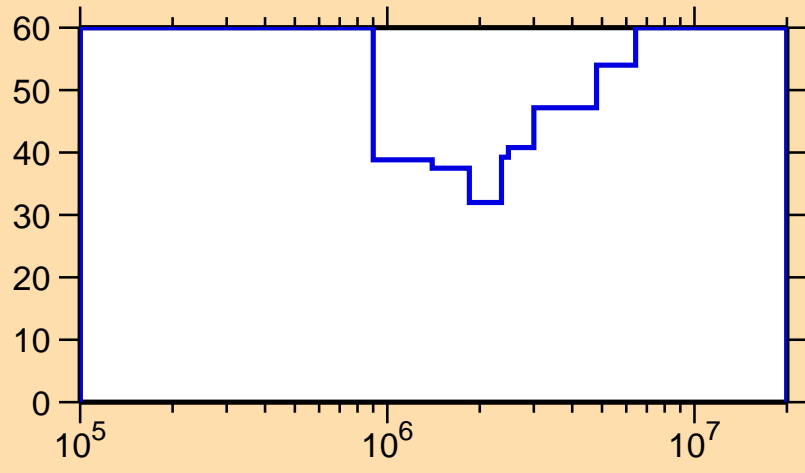
\Delta\sigma/\sigma vs. E for ^{78}\text{Y}(n,n_1)
