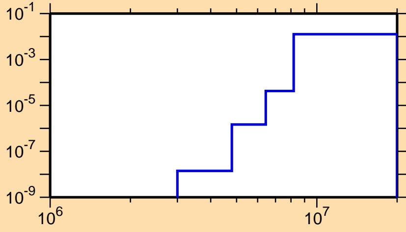
\sigma vs. E for ^{78}\text{Y}(n,\text{He}3)
