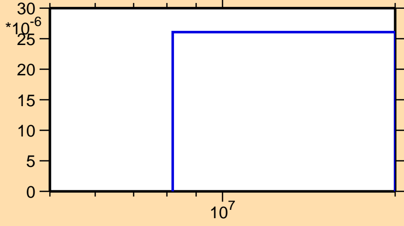
\sigma vs. E for ^{78}\text{Y}(n,\text{pt})
