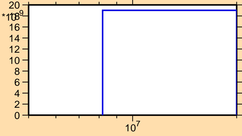
\sigma vs. E for ^{78}\text{Y}(\text{mt117})
