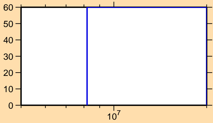
\Delta\sigma/\sigma vs. E for ^{78}\text{Y}(n,2n)
