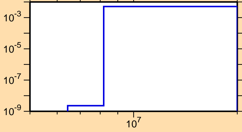
\sigma vs. E for ^{78}\text{Y}(n,\text{pd})
