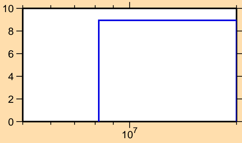
\Delta\sigma/\sigma vs. E for ^{78}\text{Y}(n,\text{nonel.})
