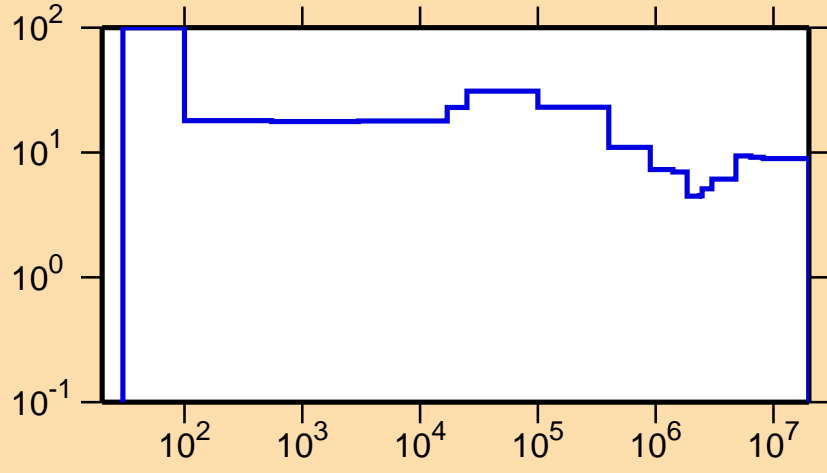
\Delta\sigma/\sigma vs. E for ^{78}\text{Y}(n,\text{nonel.})
