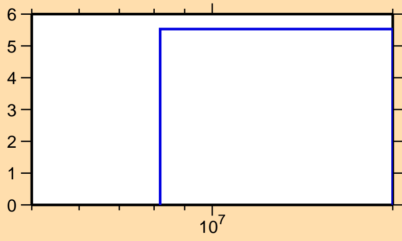
\Delta\sigma/\sigma vs. E for ^{78}\text{Y}(n,\text{el.})
