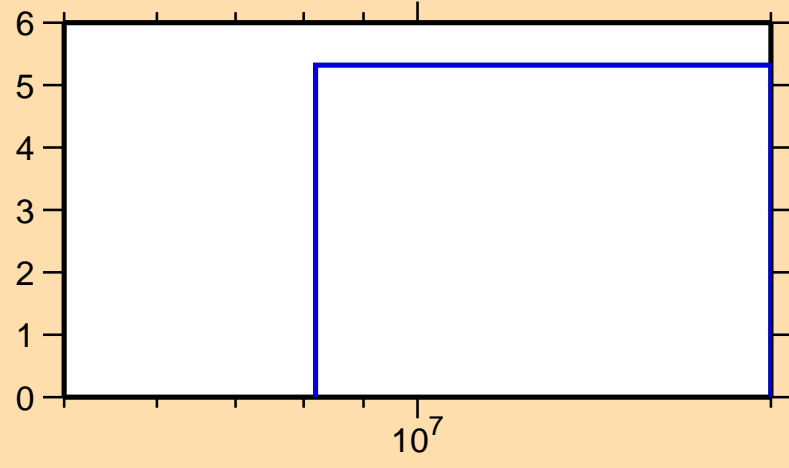
\Delta\sigma/\sigma vs. E for ^{78}\text{Y}(n,\text{tot.})
