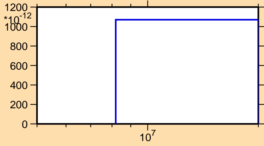
\sigma vs. E for ^{78}\text{Y} (mt 34)
