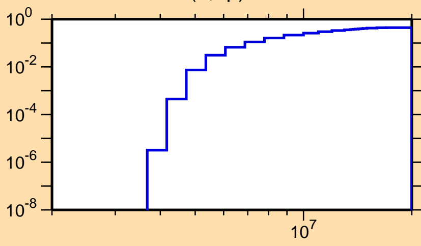
\sigma vs. E for ^{80}\text{Y}(n,np)
