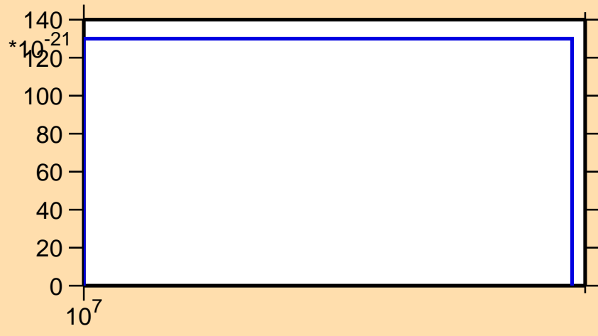
\sigma vs. E for ^{80}\text{Y}(n,nt)
