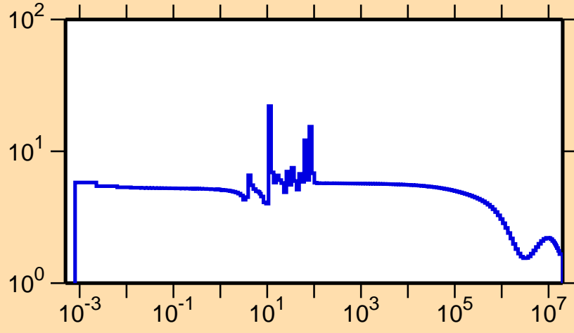
\sigma vs. E for ^{81}\text{Y}(n,\text{el.})
