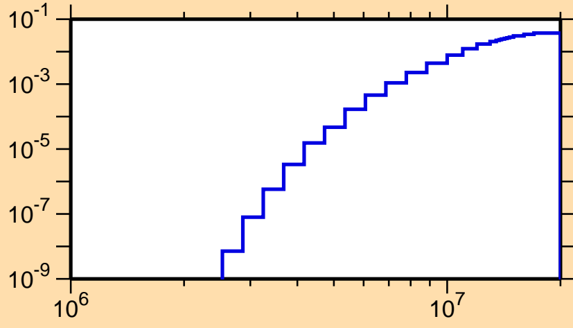
\sigma vs. E for ^{81}\text{Y}(n,d)
