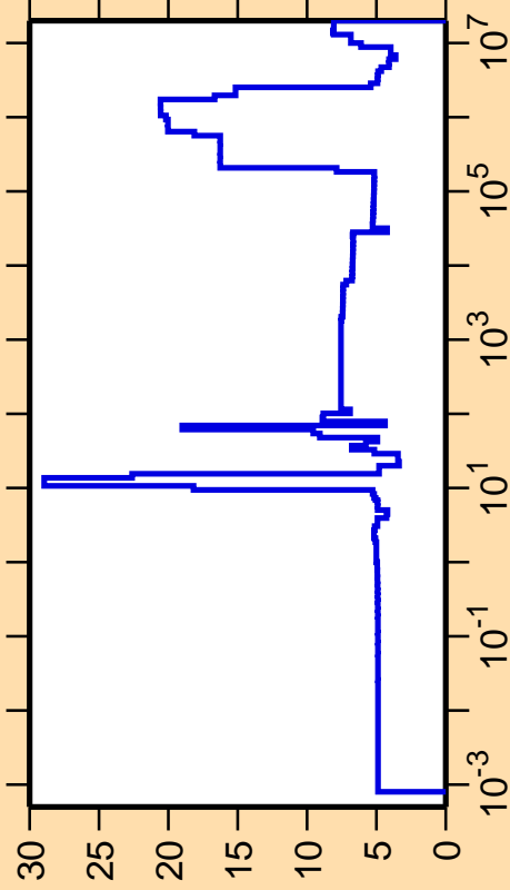
\Delta\sigma/\sigma vs. E for ^{81}\text{Y}(n,\text{el.})
