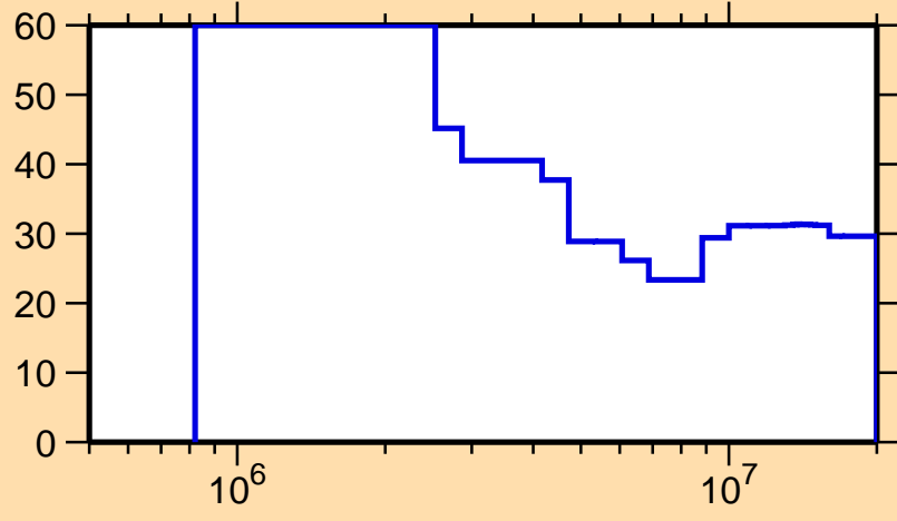
\Delta\sigma/\sigma vs. E for ^{81}\text{Y}(n,n\text{cont.})
