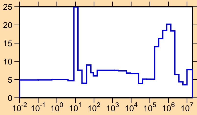
\Delta\sigma/\sigma vs. E for ^{81}\text{Y}(n,el.)
