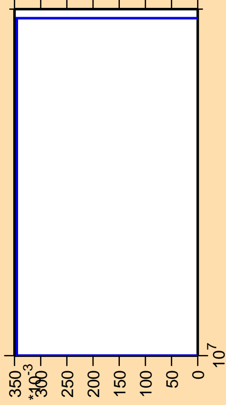
\Delta\sigma/\sigma vs. E for ^{81}\text{Y} (mt 34)
