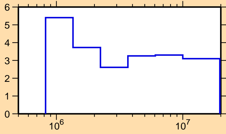
\Delta\sigma/\sigma vs. E for ^{81}\text{Y}(n,n\text{onel.})
