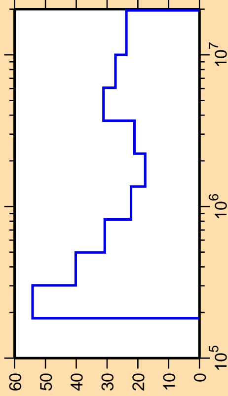
\Delta\sigma/\sigma vs. E for ^{82}\text{Y}(n,n_2)
