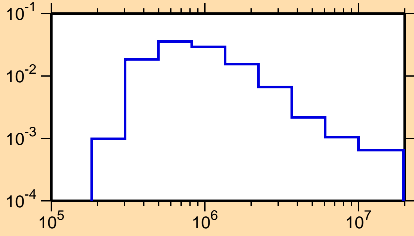
\sigma vs. E for ^{82}\text{Y}(n,n_2)
