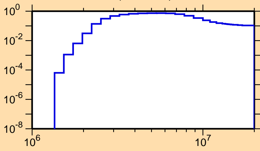
\sigma vs. E for ^{83}\text{Y}(n,n\text{cont.})
