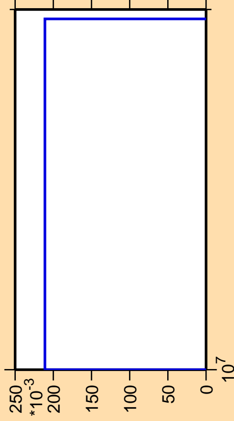
\Delta\sigma/\sigma vs. E for ^{83}\text{Y}(n,nt)
