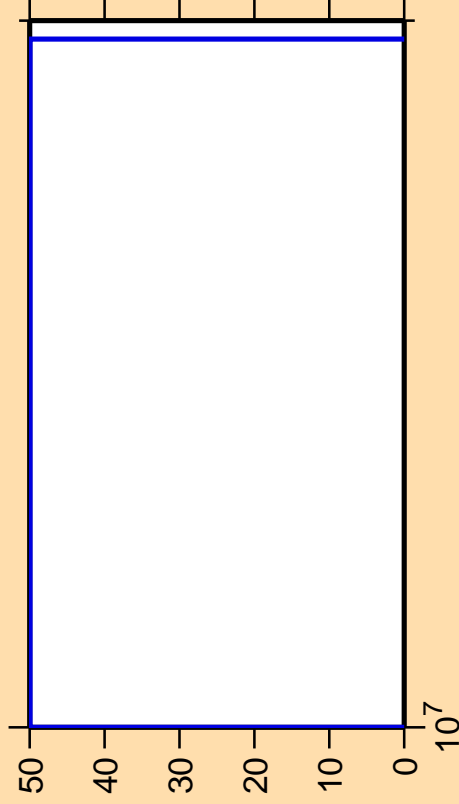
\Delta\sigma/\sigma vs. E for ^{83}\text{Y}(n,nd)
