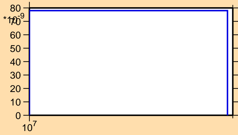
\sigma vs. E for ^{83}\text{Y}(n,nd)
