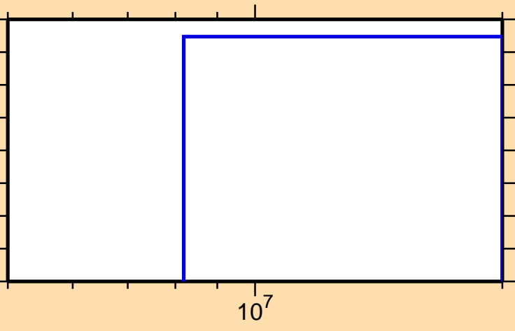
\sigma vs. E for ^{83}\text{Y}(n,2n)
