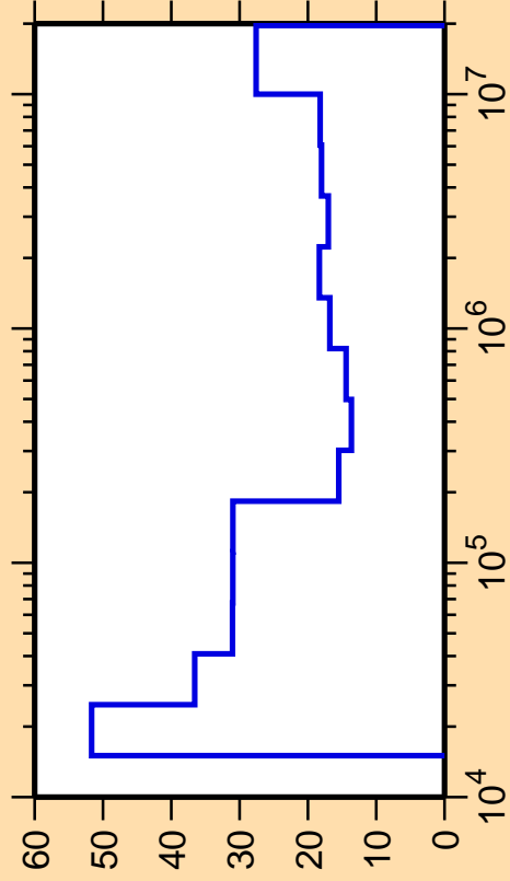
\Delta\sigma/\sigma vs. E for ^{84}\text{Y}(n,n_1)
