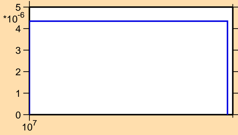
\sigma vs. E for ^{84}\text{Y}(n,\text{nd})
