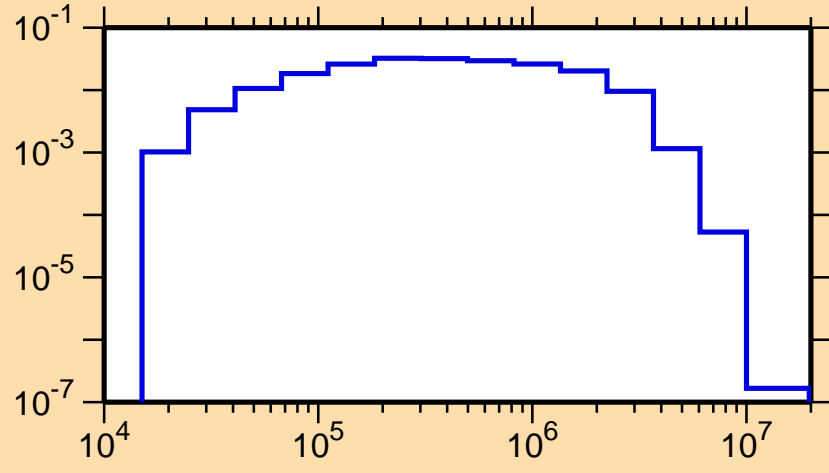
\sigma vs. E for ^{84}\text{Y}(n,n_1)
