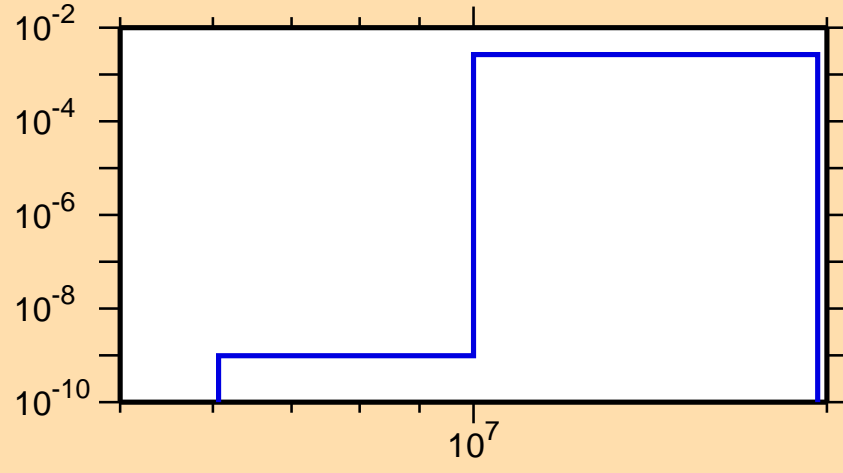
\sigma vs. E for ^{84}\text{Y}(n,n\alpha)
