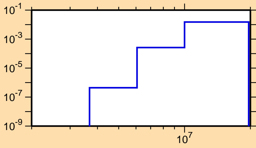
\sigma vs. E for ^{84}\text{Y}(n,d)
