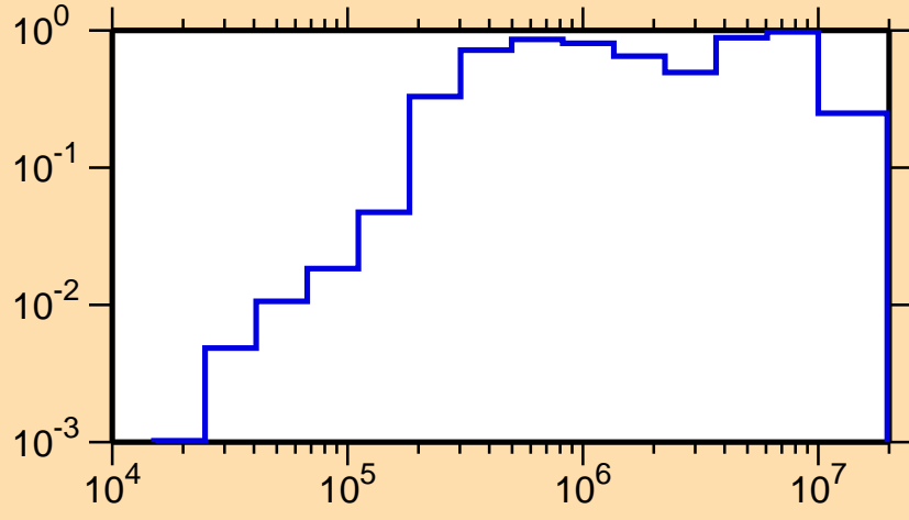
\sigma vs. E for ^{84}\text{Y}(n,\text{inel.})
