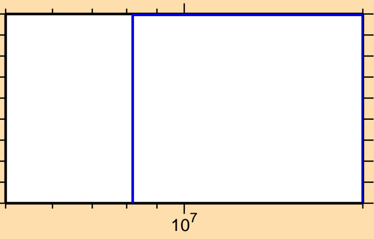
\sigma vs. E for ^{84}\text{Y}(n,\text{He}3)
