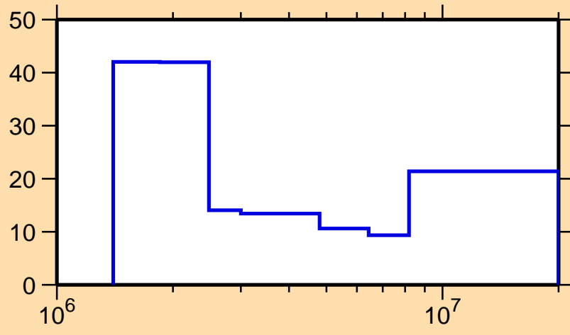
\Delta\sigma/\sigma vs. E for ^{84}\text{Y}(n,ncont.)
