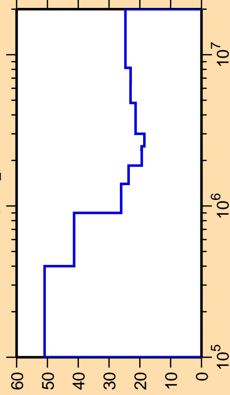
\Delta\sigma/\sigma vs. E for ^{84}\text{Y}(n,n_2)
