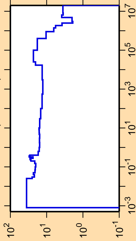
\Delta\sigma/\sigma vs. E for ^{84}\text{Y}(n,\text{nonel.})
